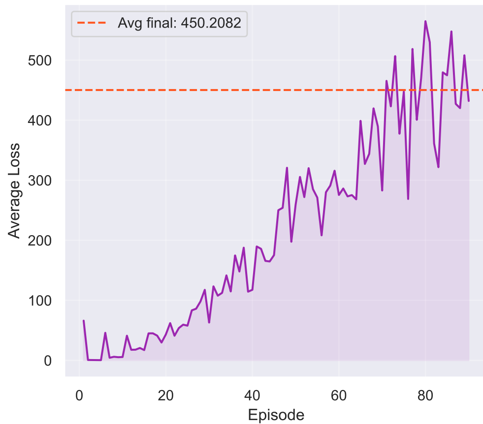
DQN Training: Loss vs Episodes
