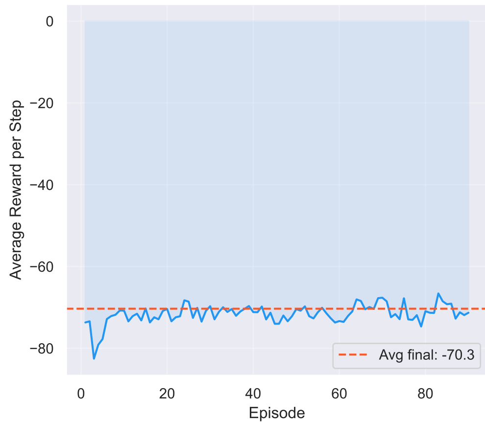
DQN Training: Reward vs Episodes
