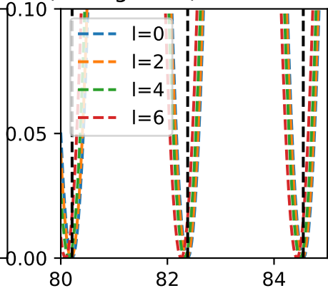
CPA at large kR (even TM modes)
