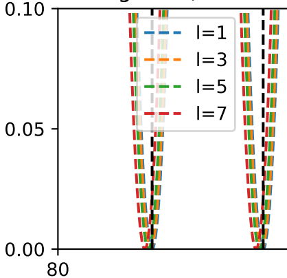
CPA at large kR (odd TE modes)
