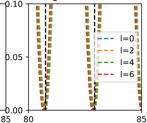
CPA at large kR (even TE modes)
