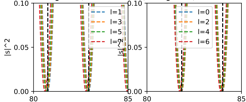
CPA at large kR (odd TM modes)
