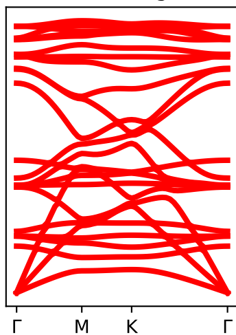
Buckling
