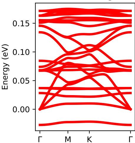
No Buckling
