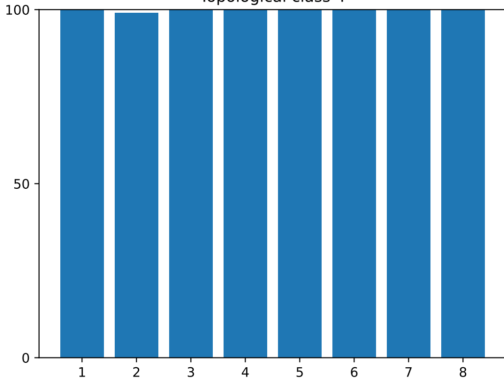
Topological class 4
