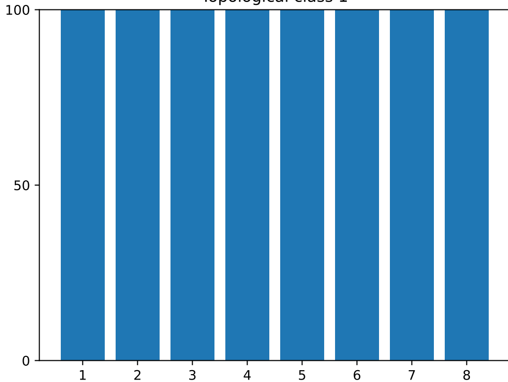
Topological class 1
