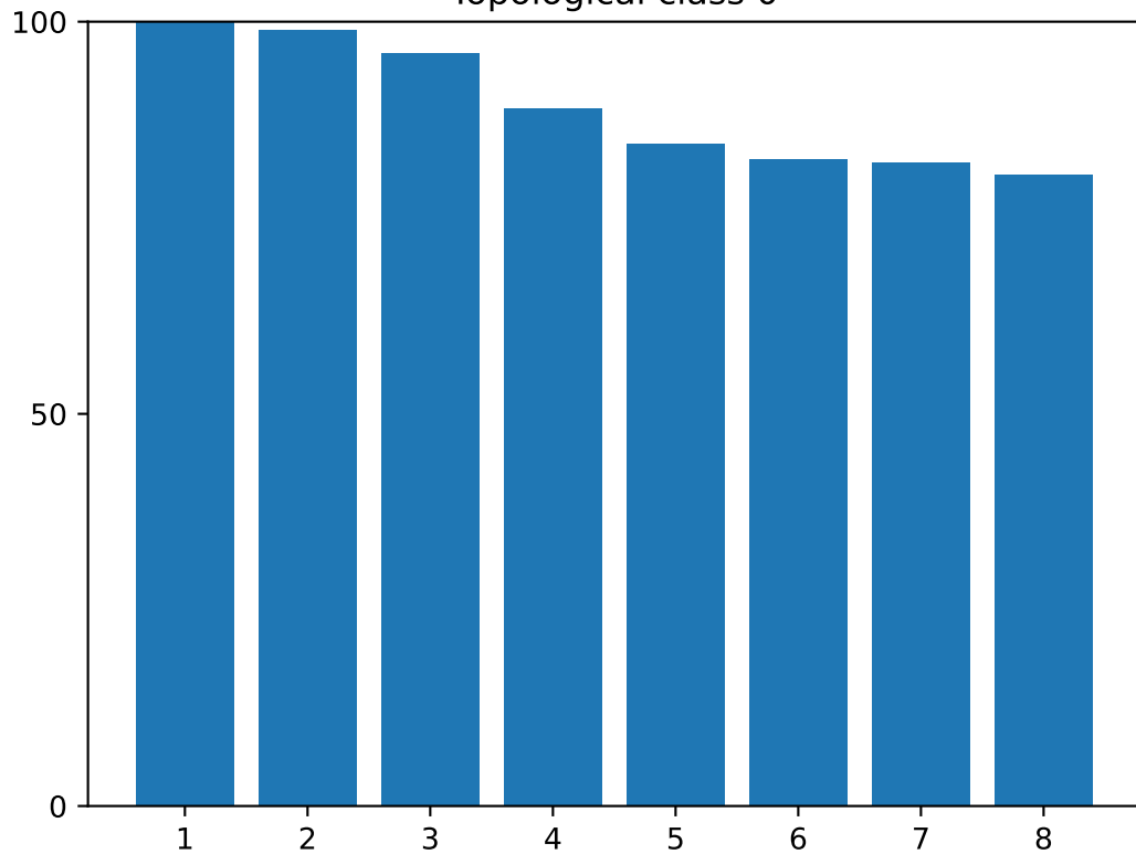
Topological class 0
