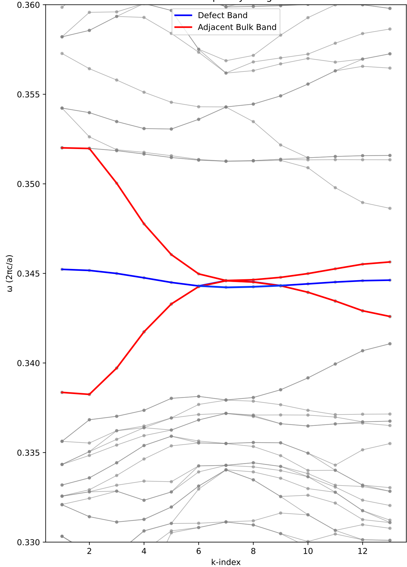
Band Structure - Frequency Range 0.33 to 0.36
