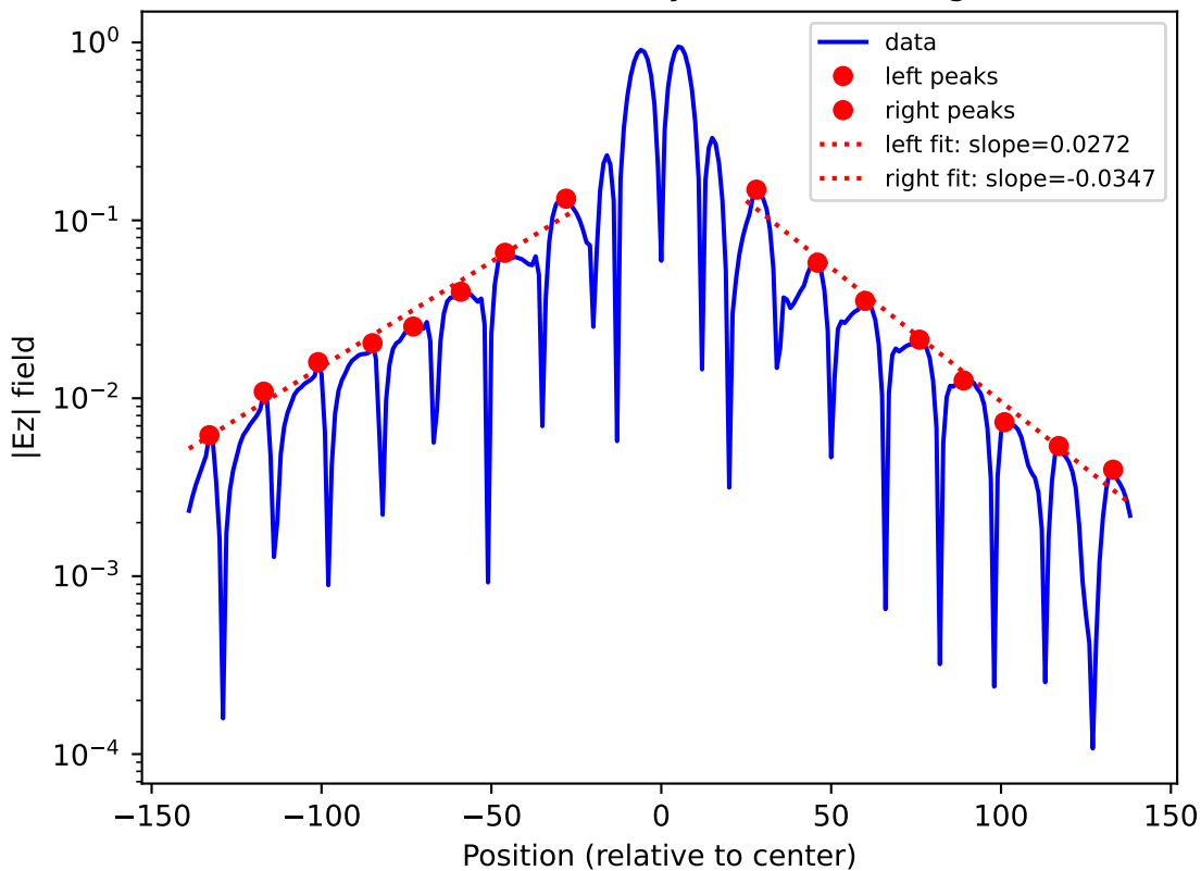
Line cut at z=248, y=248 (semi-log)
