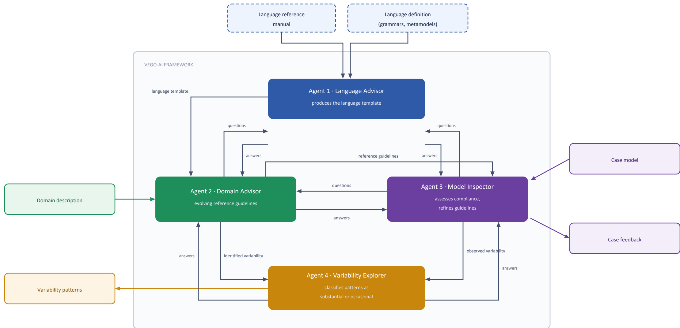
Figure 1. The VEGO-AI four-agent architecture.
