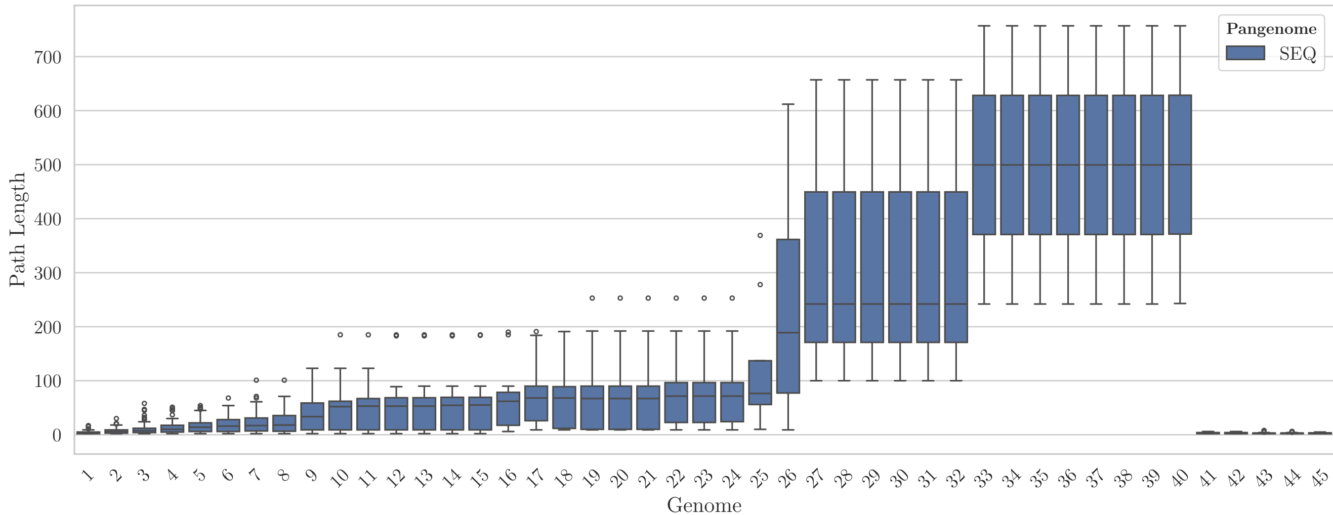
Path Length Distribution per Genome
