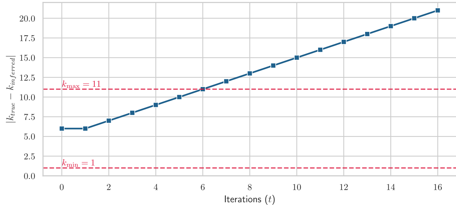
Genome Count Tracking: Edge Assignment ( \alpha = 0.5, \gamma = 1.0 )
