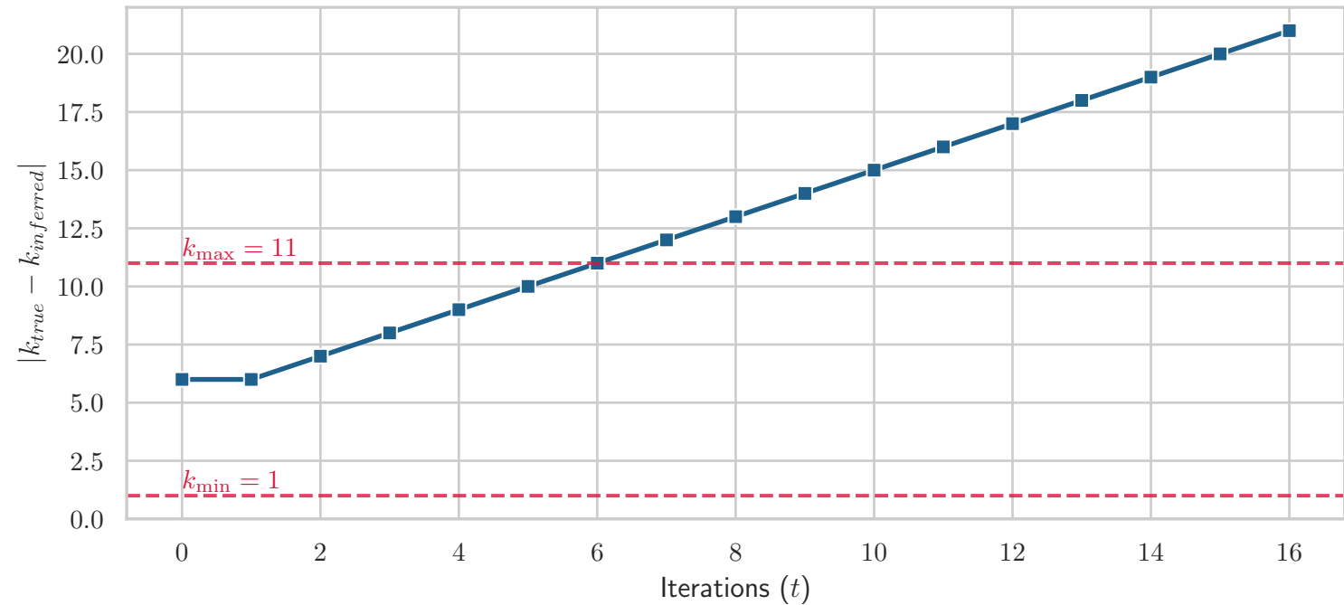
Genome Count Tracking: Edge Assignment ( \alpha = 1.0, \gamma = 1.0 )
