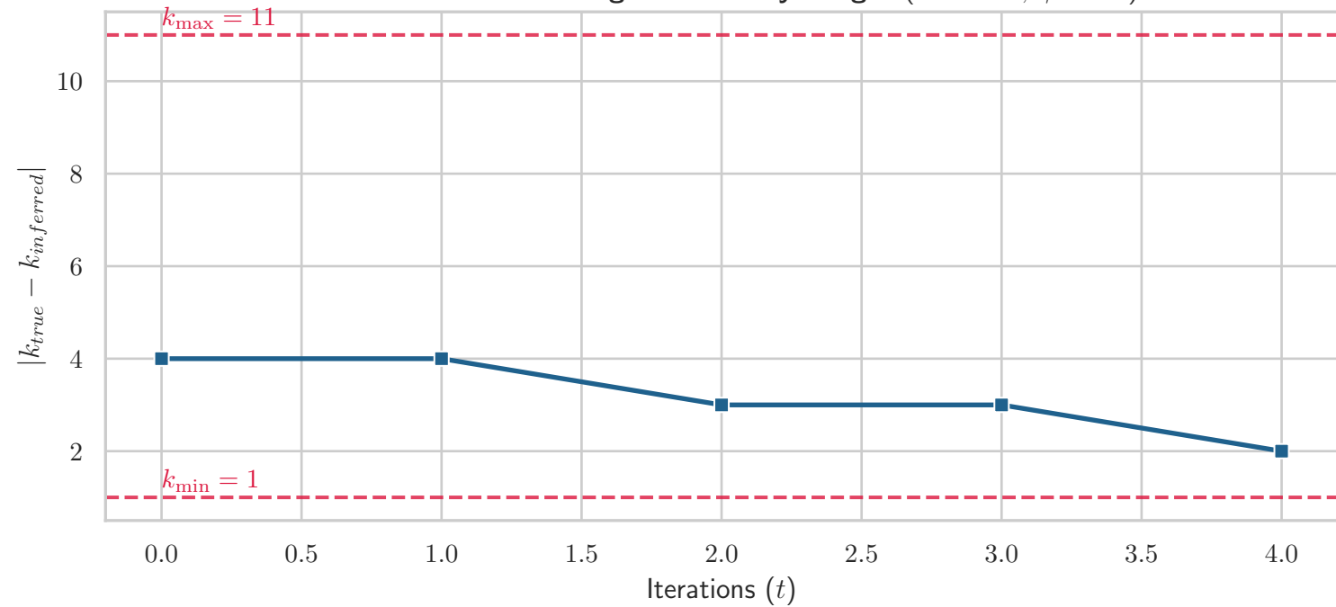
Genome Count Tracking: Eulerian by Length ( \alpha = 0.25 , \gamma = 1.0 )
