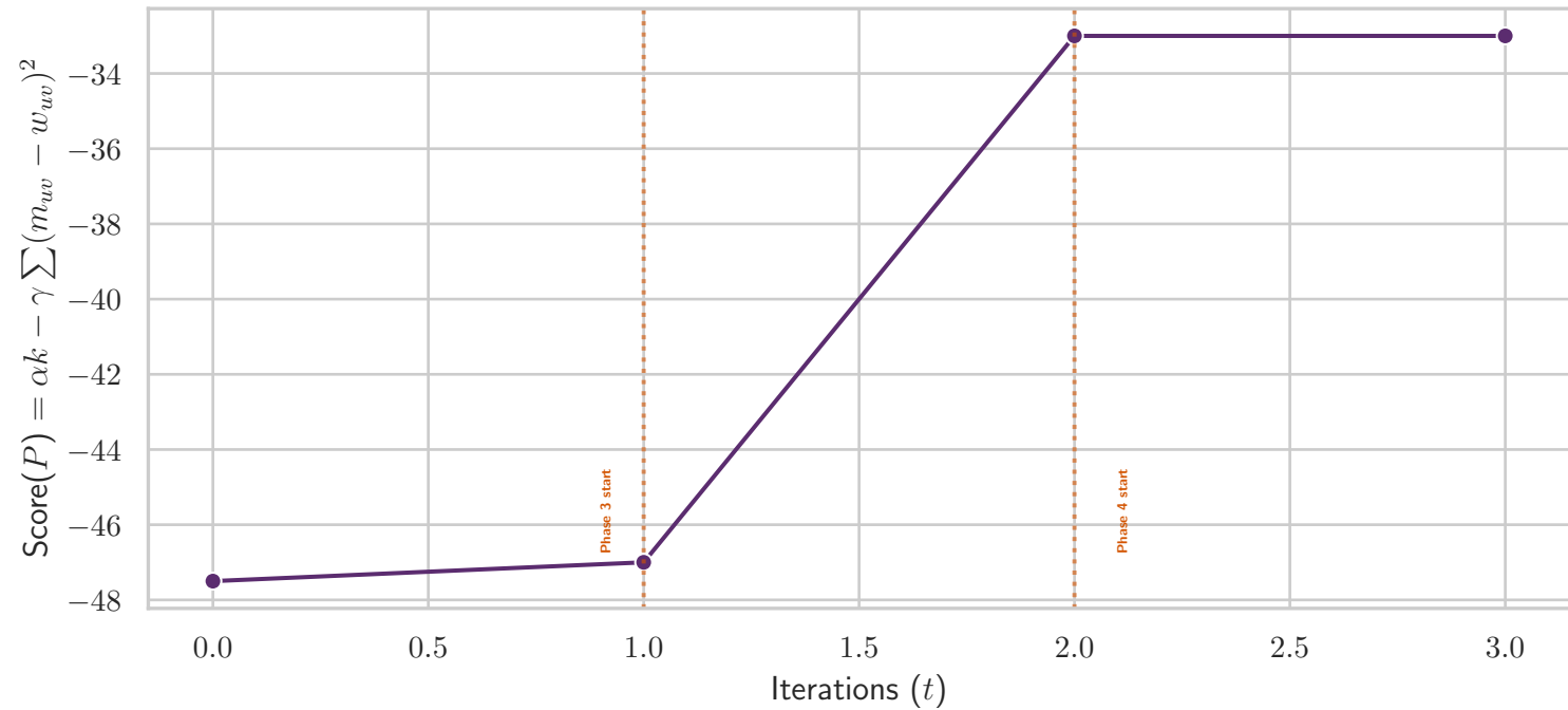
Score Tracking: Eulerian by Length ( \alpha = 0.5, \gamma = 1.0 )
