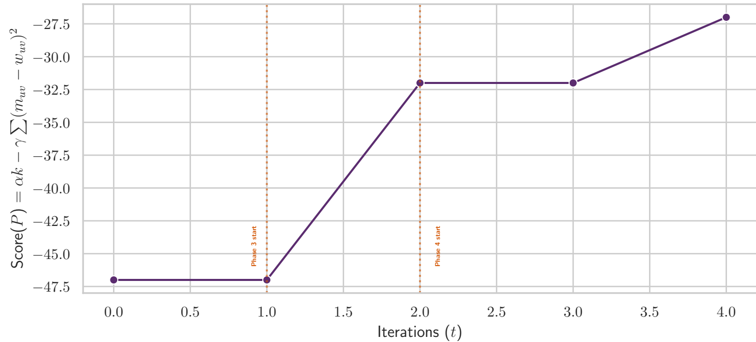
Score Tracking: Eulerian by Length ( \alpha = 1.0, \gamma = 1.0 )
