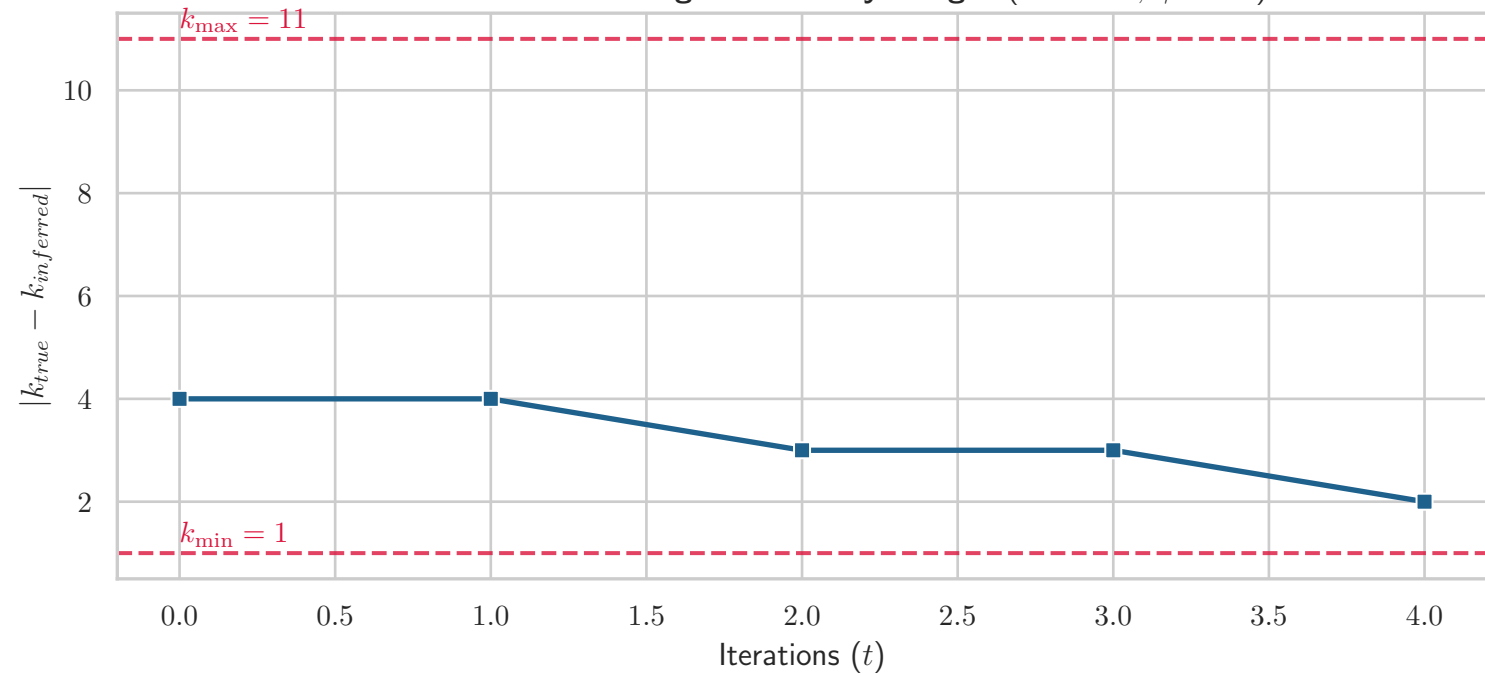
Genome Count Tracking: Eulerian by Weight ( \alpha = 0.25, \gamma = 1.0 )
