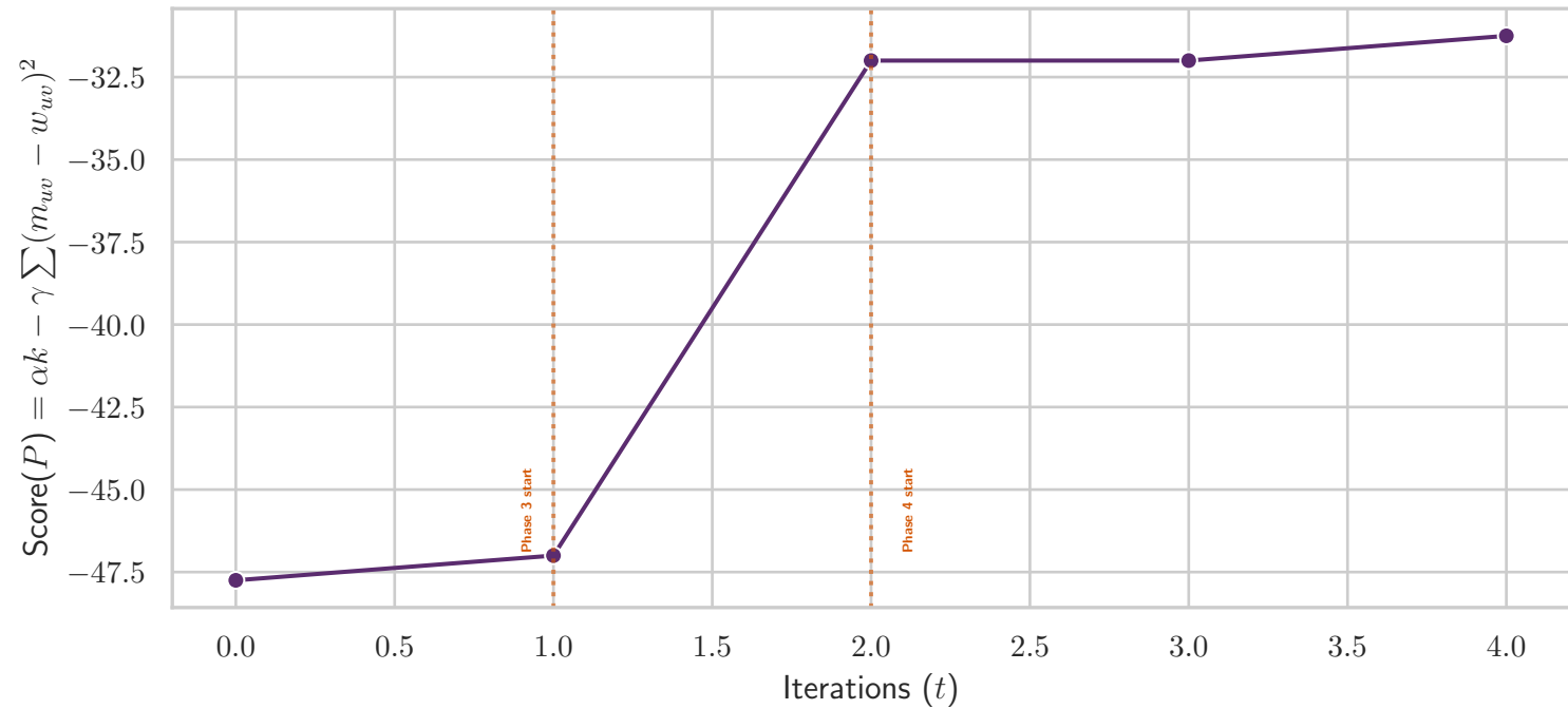
Score Tracking: Eulerian by Weight ( \alpha = 0.25, \gamma = 1.0 )
