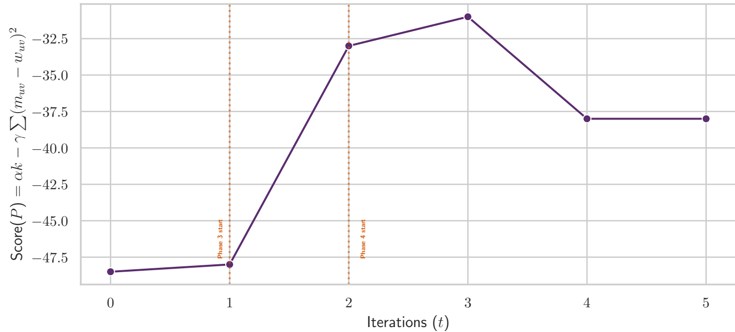
Score Tracking: Eulerian by Weight ( \alpha = 0.5, \gamma = 1.0 )
