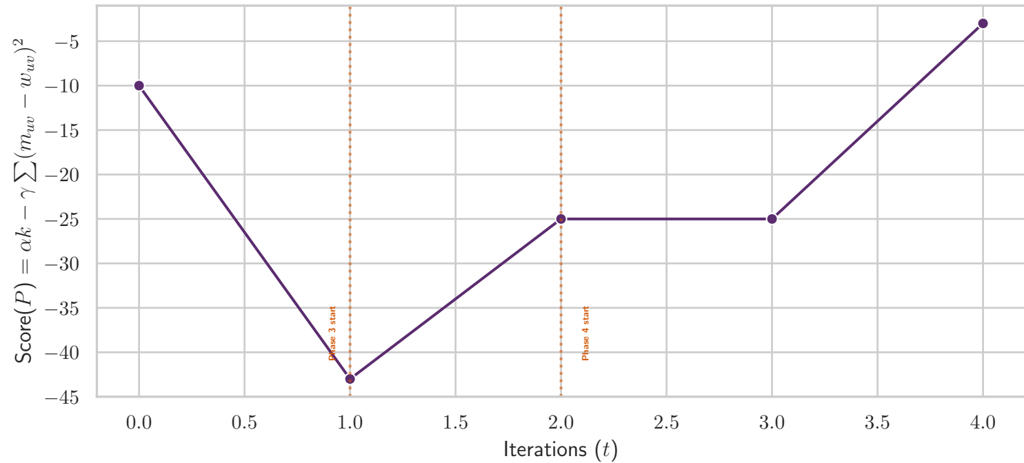
Score Tracking: Eulerian by Weight ( \alpha = 1.0, \gamma = 0.25 )
