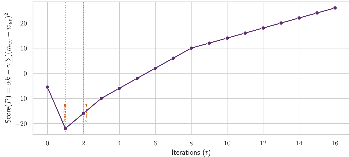
Score Tracking: Edge Assignment ( \alpha = 1.0, \gamma = 0.5 )
