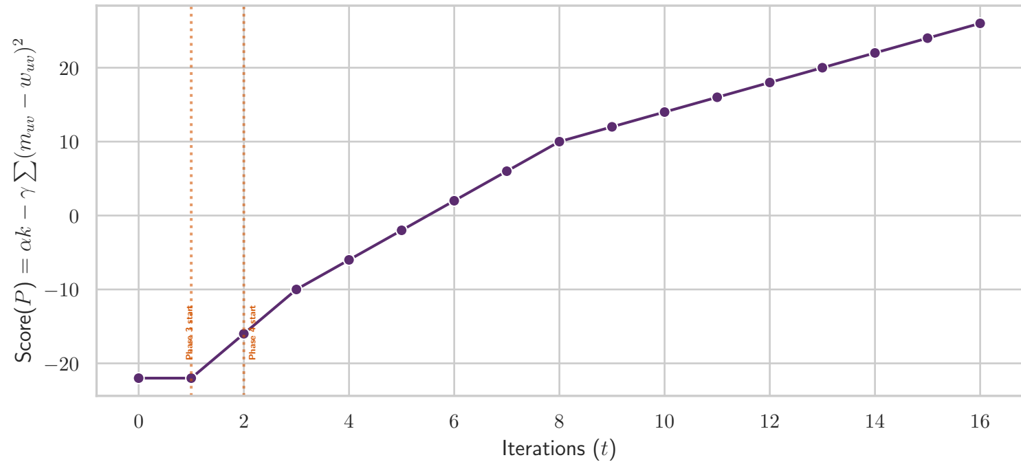
Score Tracking: Edge Assignment ( \alpha = 1.0, \gamma = 1.0 )
