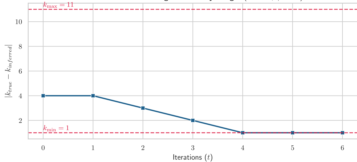
Genome Count Tracking: Eulerian by Weight ( \alpha = 1.0 , \gamma = 0.5 )
