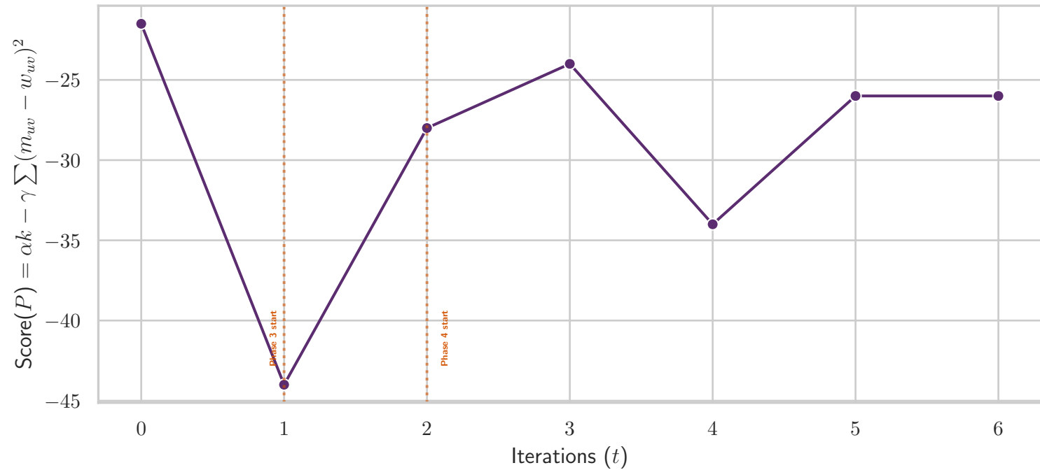
Score Tracking: Eulerian by Weight ( \alpha = 1.0, \gamma = 0.5 )
