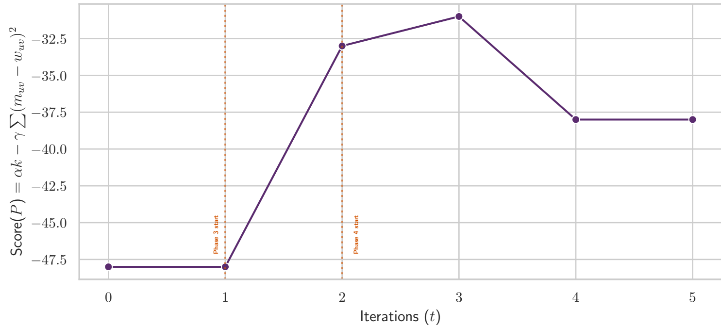
Score Tracking: Eulerian by Weight ( \alpha = 1.0, \gamma = 1.0 )
