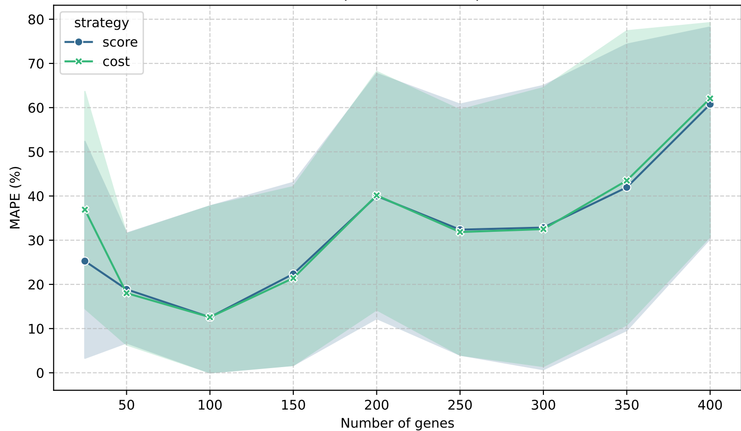
MAPE Comparison ( \alpha=1.0 , \gamma=0.25 )
