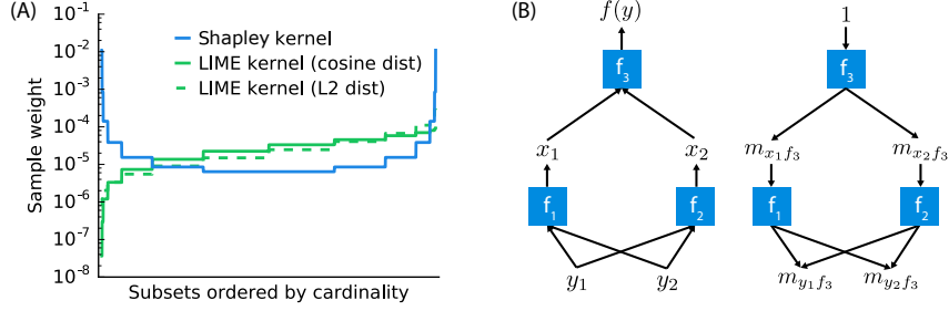
Figure 2: (A) The Shapley kernel weighting is symmetric when all possible \mathbf{z}' vectors are ordered by cardinality there are 2^{15} vectors in this example. This is distinctly different from previous heuristically chosen kernels. (B) Compositional models such as deep neural networks are comprised of many simple components. Given analytic solutions for the Shapley values of the components, fast approximations for the full model can be made using DeepLIFT’s style of back-propagation.
