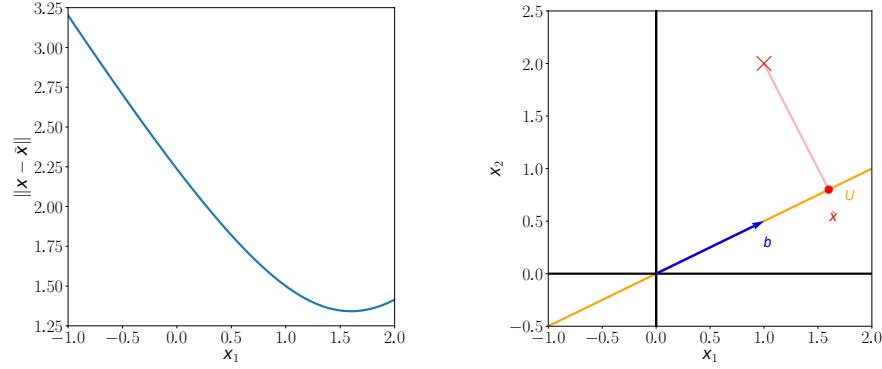
Figure 10.8 Optimal projection of a vector \mathbf{x} \in \mathbb{R}^2 onto a one-dimensional subspace (continuation from Figure 10.7). (a) Distances \|\mathbf{x} - \tilde{\mathbf{x}}\| for some \mathbf{x} \in U . (b) Orthogonal projection and optimal coordinates.
