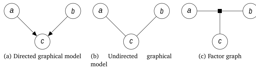
Figure 8.12 Three types of graphical models: (a) Directed graphical models (Bayesian networks); (b) Undirected graphical models (Markov random fields); (c) Factor graphs.
