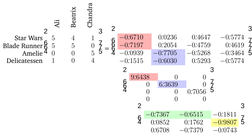
Figure 4.10 Movie ratings of three people for four movies and its SVD decomposition.
