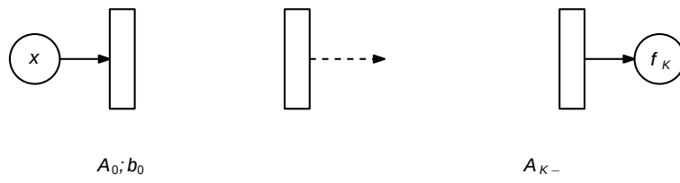
Figure 5.8 Forward pass in a multi-layer neural network to compute the loss L as a function of the inputs \mathbf{x} and the parameters \mathbf{A}_i, \mathbf{b}_i .
