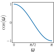
Figure 3.4 When restricted to [0; \pi] then f(!) = \cos(!) returns a unique number in the interval [-1; 1] .
