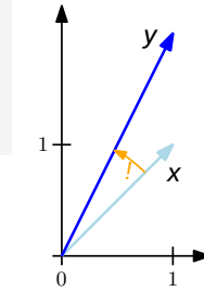
Figure 3.5 The angle \theta between two vectors \mathbf{x}; \mathbf{y} is computed using the inner product.
