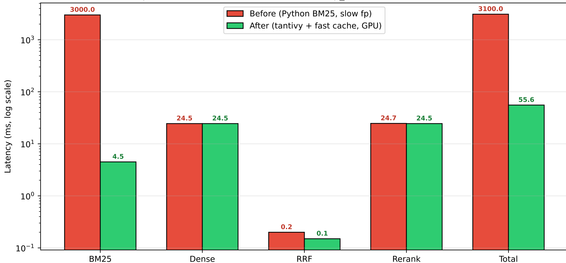
Latency Breakdown: Before vs After (warm, top_k=5, 1405-07-06, 1110 chunks)
