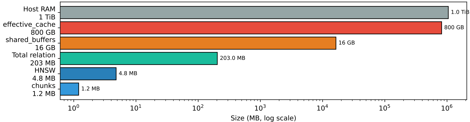
Postgres Vectors Fit Entirely in RAM (pg_prewarm 750 blocks)
