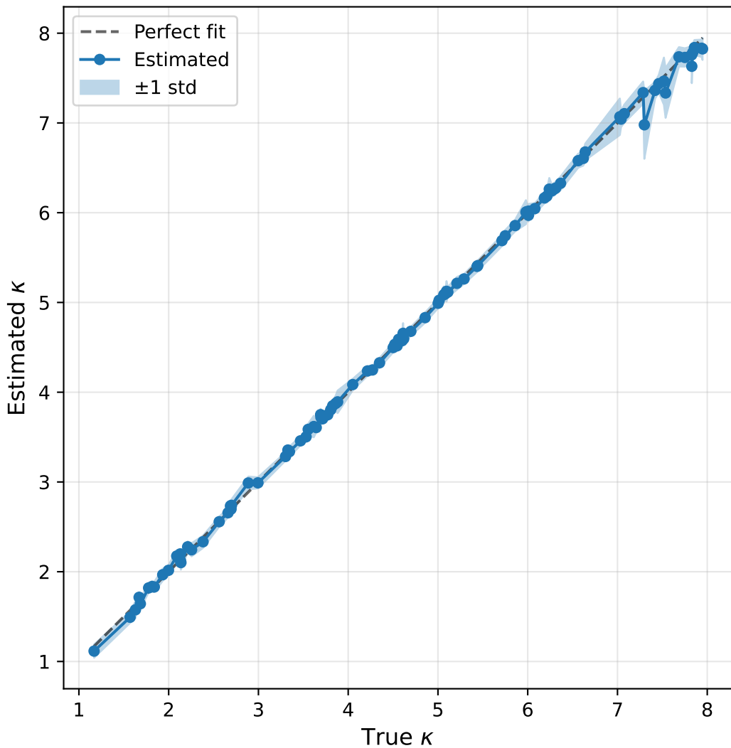
\kappa : True vs Estimated
