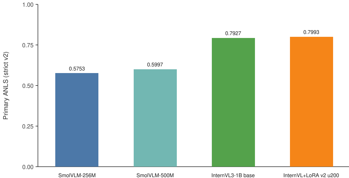
Holdout primary ANLS (n=504)
