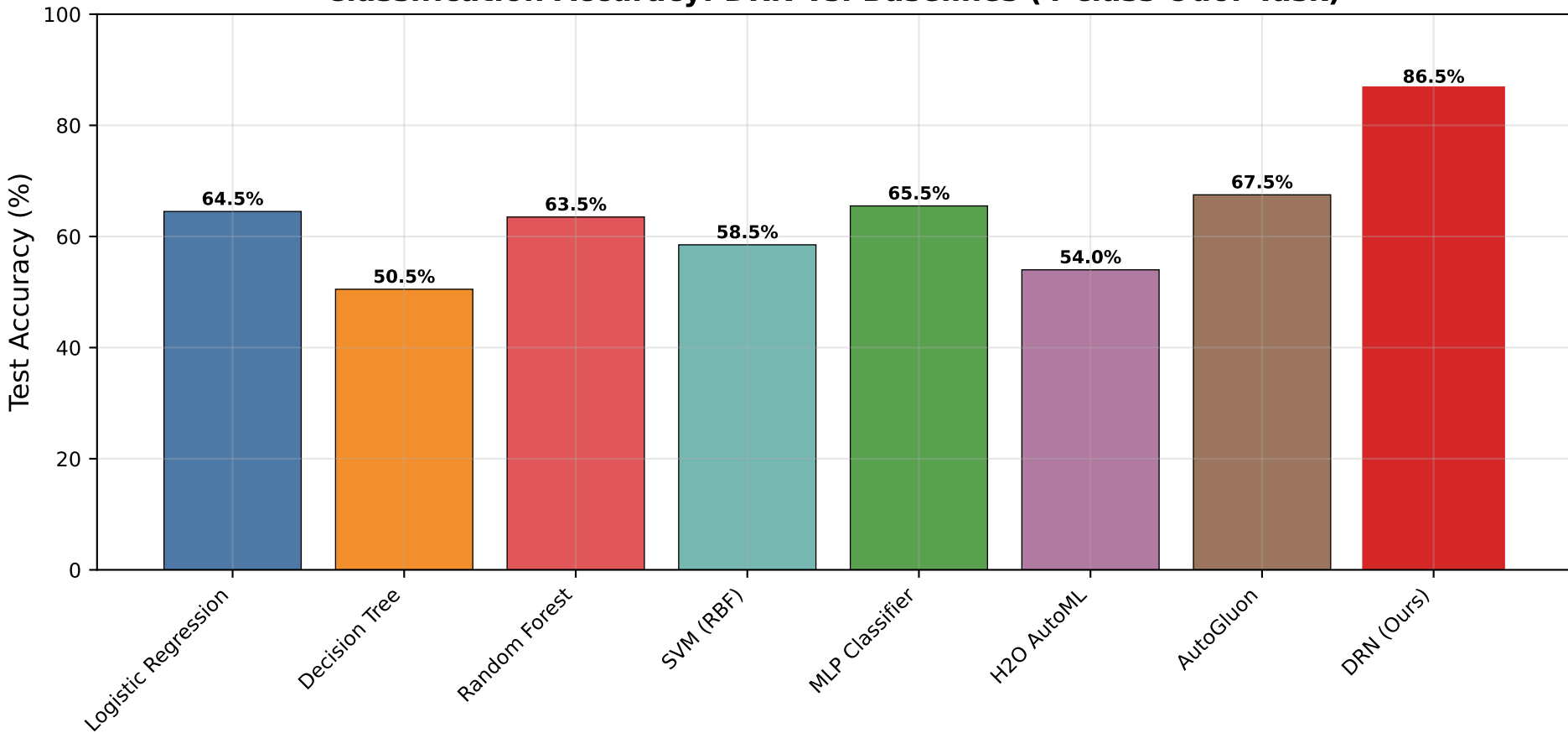
Classification Accuracy: DRN vs. Baselines (4-class Odor Task)
