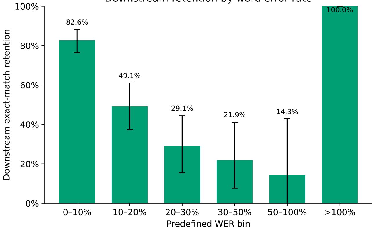
Downstream retention by word error rate
