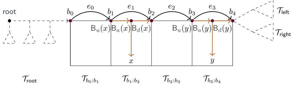
Figure 5 Partitioning a branch of a tree \mathcal{T} using a bough B . Here, the nodes b_i for 0 \leq i \leq 4 are k -neighbours forming the backbone B . The letter e_i denotes idempotent monoid element \llbracket b_i : b_{i+1} \rrbracket_{\mathcal{T}} . In dashed, we represented the context C[\square] such that \mathcal{T} = C[B] . To compute the presence of an edge between x and y in the resulting graph, it is sufficient to know the values of \llbracket b_2 : b_3 \rrbracket_{\mathcal{T}} , and the respective bough types of x and y in their respective bough blocks \mathcal{T}_{b_1:b_2} and \mathcal{T}_{b_3:b_4} .
