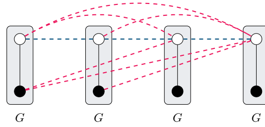
■ Figure 6 The graph S_4 as described in Example 36. The dashed edges represents the edges defined by C and F , respectively in blue and in red. Vertices originating from the same copy of G are grouped in rectangles.
