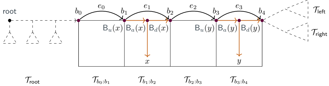
Figure 5 Partitioning a branch of a tree \mathcal{T} using a bough B . Here, the nodes b_i for 0 \leq i \leq 4 are k -neighbours forming the backbone B . The letter e_i denotes idempotent monoid element \llbracket b_i : b_{i+1} \rrbracket_{\mathcal{T}} . In dashed, we represented the context C[\square] such that \mathcal{T} = C[B] . To compute the presence of an edge between x and y in the resulting graph, it is sufficient to know the values of \llbracket b_2 : b_3 \rrbracket_{\mathcal{T}} , and the respective bough types of x and y in their respective bough blocks \mathcal{T}_{b_1:b_2} and \mathcal{T}_{b_3:b_4} .
