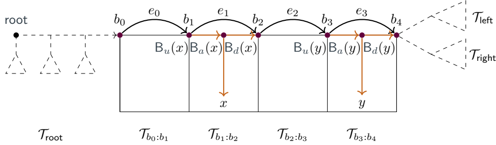
Figure 5 Partitioning a branch of a tree \mathcal{T} using a bough B . Here, the nodes b_i for 0 \leq i \leq 4 are k -neighbours forming the backbone B . The letter e_i denotes idempotent monoid element \llbracket b_i : b_{i+1} \rrbracket_{\mathcal{T}} . In dashed, we represented the context C[\square] such that \mathcal{T} = C[B] . To compute the presence of an edge between x and y in the resulting graph, it is sufficient to know the values of \llbracket b_2 : b_3 \rrbracket_{\mathcal{T}} , and the respective bough types of x and y in their respective bough blocks \mathcal{T}_{b_1:b_2} and \mathcal{T}_{b_3:b_4} .
