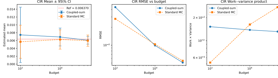
Figure 3: CIR option pricing. Left: mean with 95% CI. Centre: RMSE vs budget. Right: work-variance product. Coupled-sum (circles) vs standard MC (squares).
