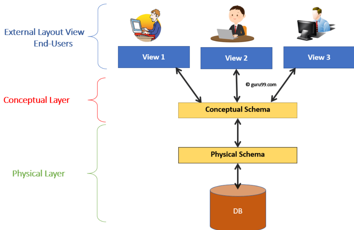
ANSI_SPARC Architecture of the database system
