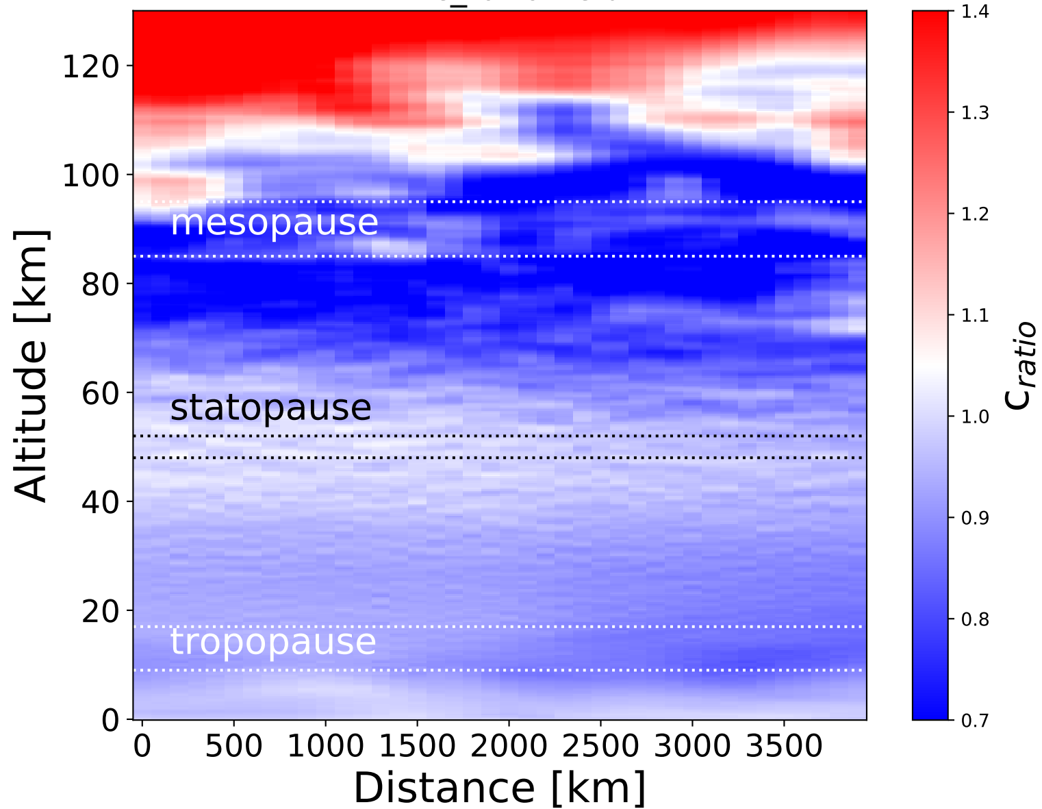
2D c_ratio field
