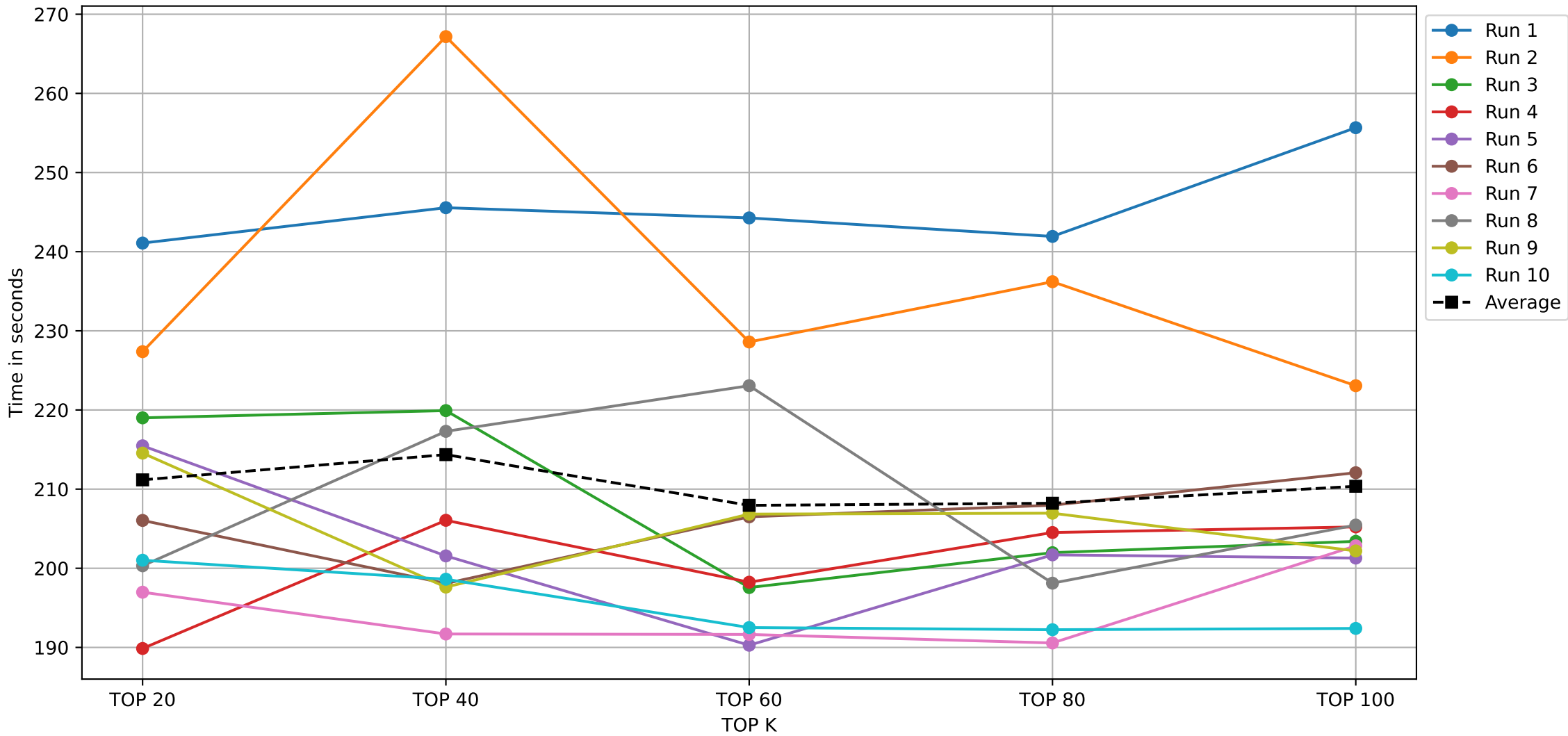
USER DEFINE ALGORITHM ON 2,000,000 TRANSACTIONS DATABASE
