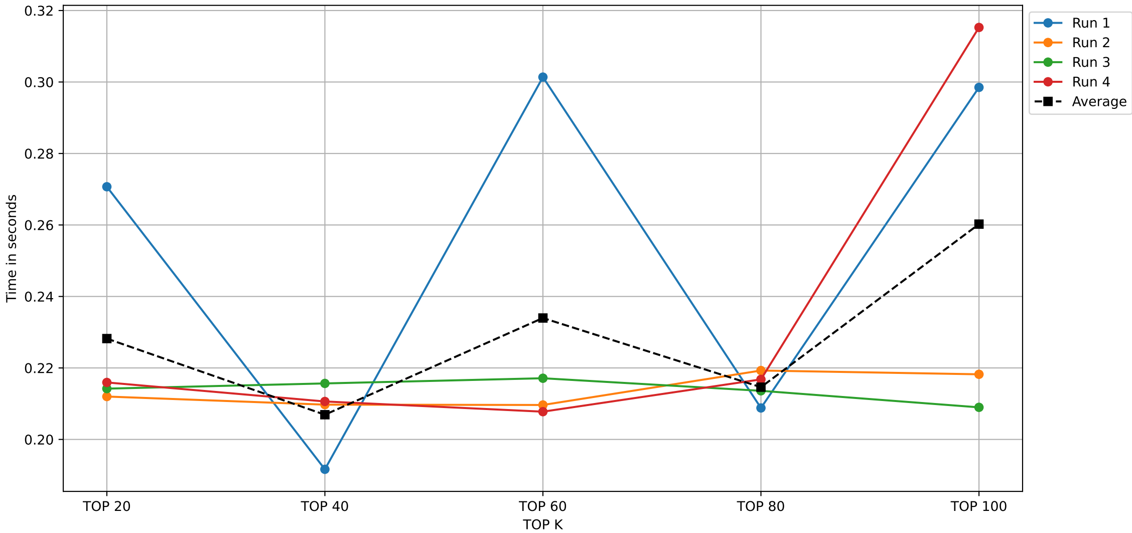
USER DEFINE ALGORITHM ON 5,000 TRANSACTIONS DATABASE
