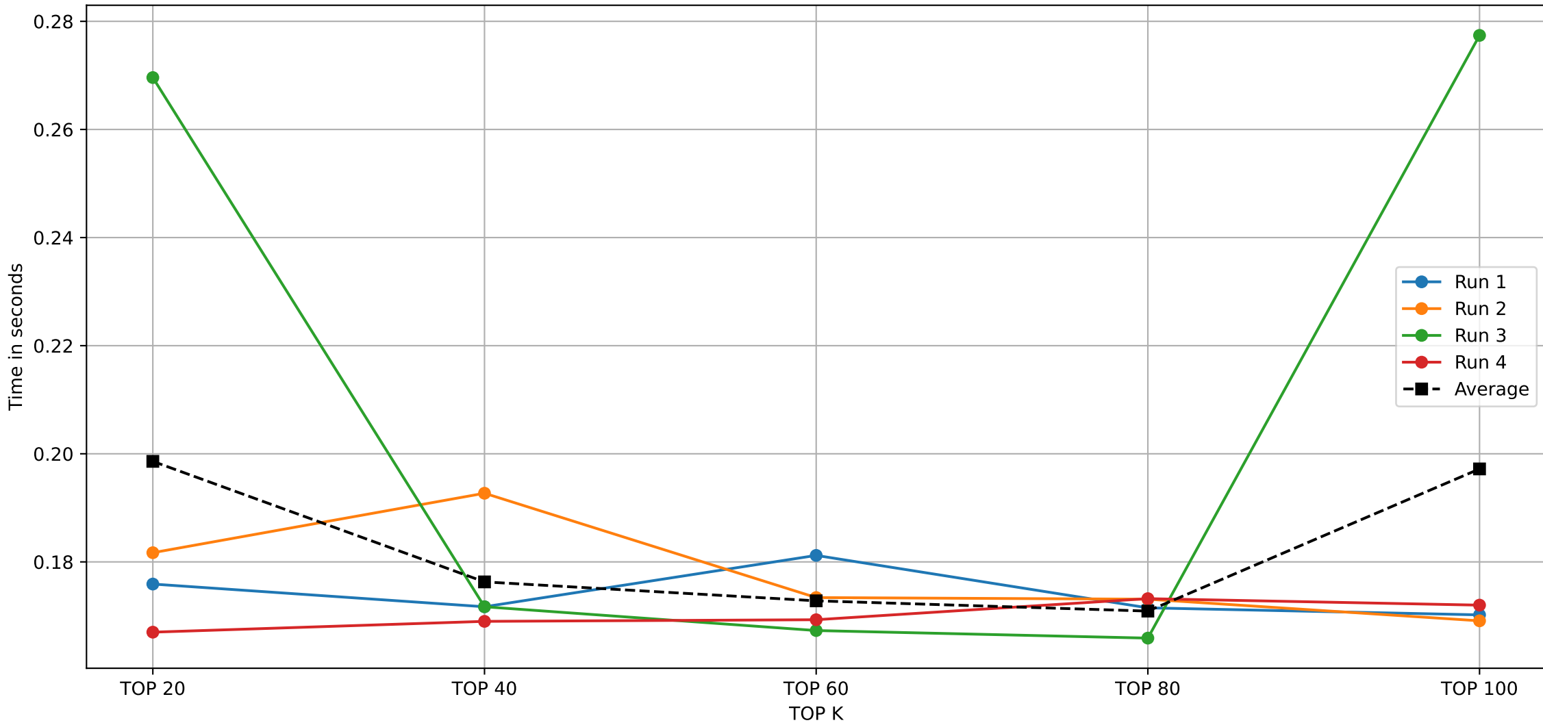
HEURISTIC ALGORITHM ON 2000 TRANSACTIONS DATABASE
