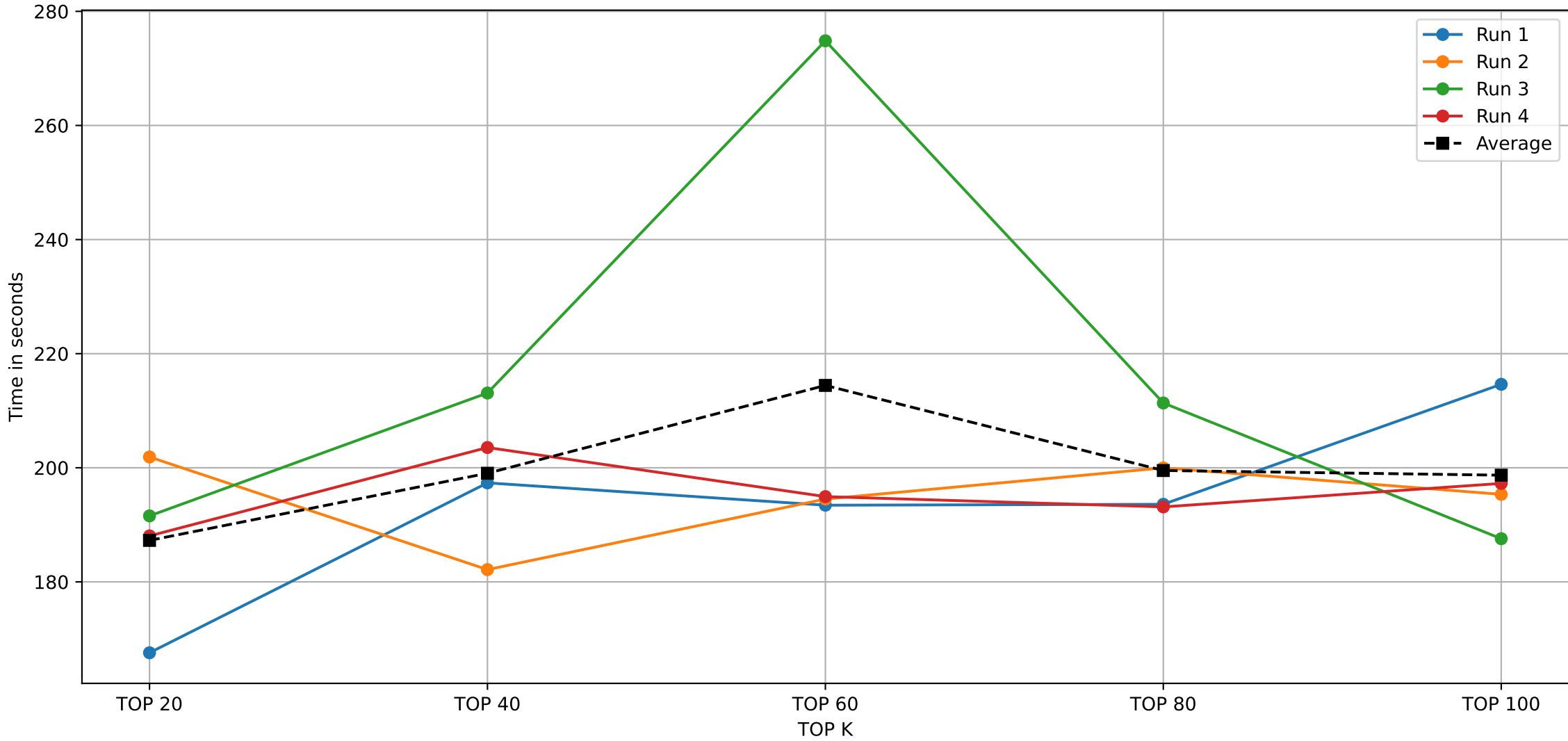
NAIVE ALGORITHM ON 2000000 TRANSACTIONS DATABASE
