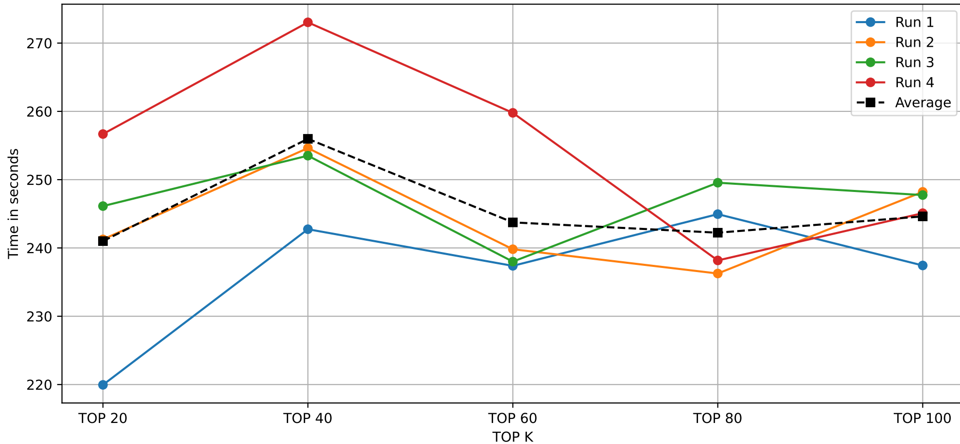
HEURISTIC ALGORITHM ON DATABASE_2000000
