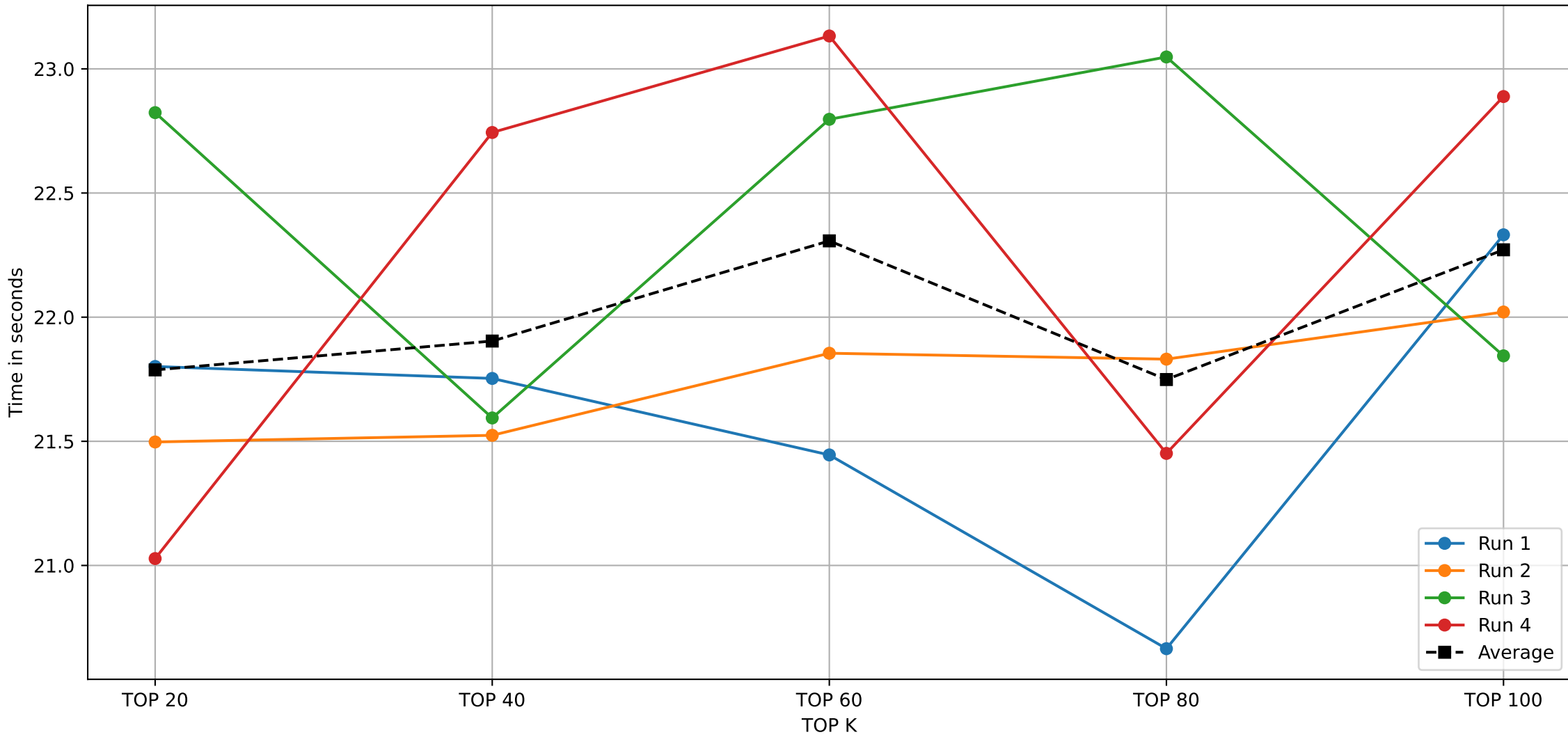
NAIVE ALGORITHM ON 200000 TRANSACTIONS DATABASE
