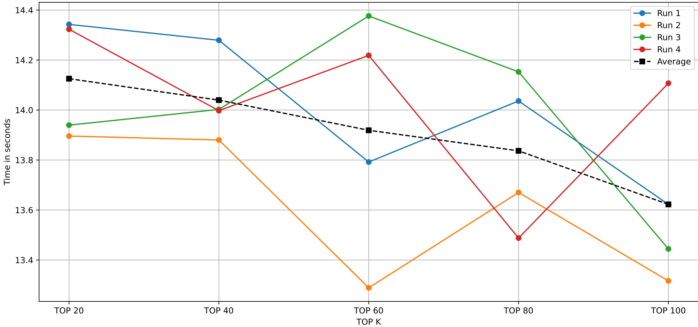
HEURISTIC ALGORITHM ON 100000 TRANSACTIONS DATABASE
