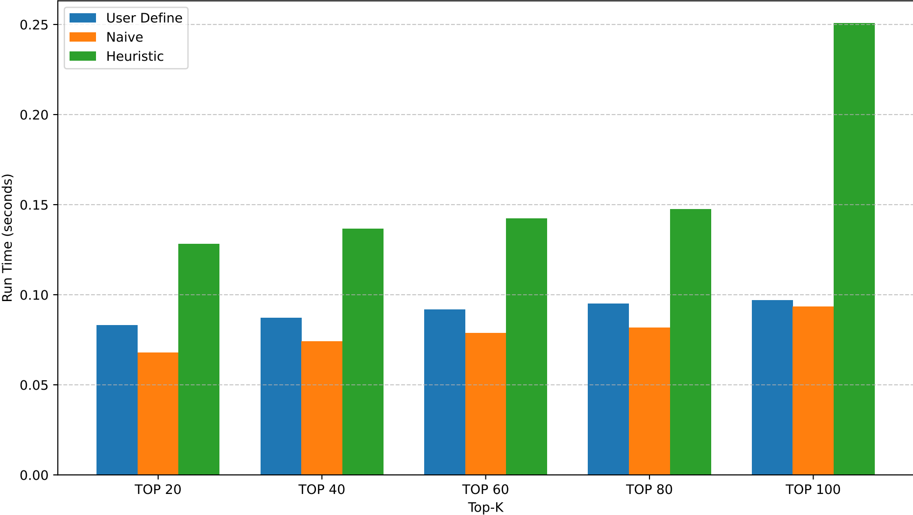
Run Time Comparison (1000 Transactions)
