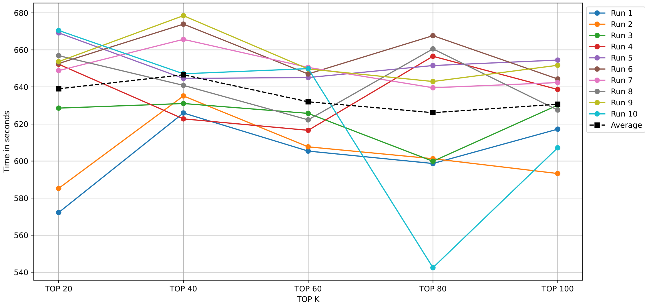
USER DEFINE ALGORITHM ON 5,000,000 TRANSACTIONS DATABASE
