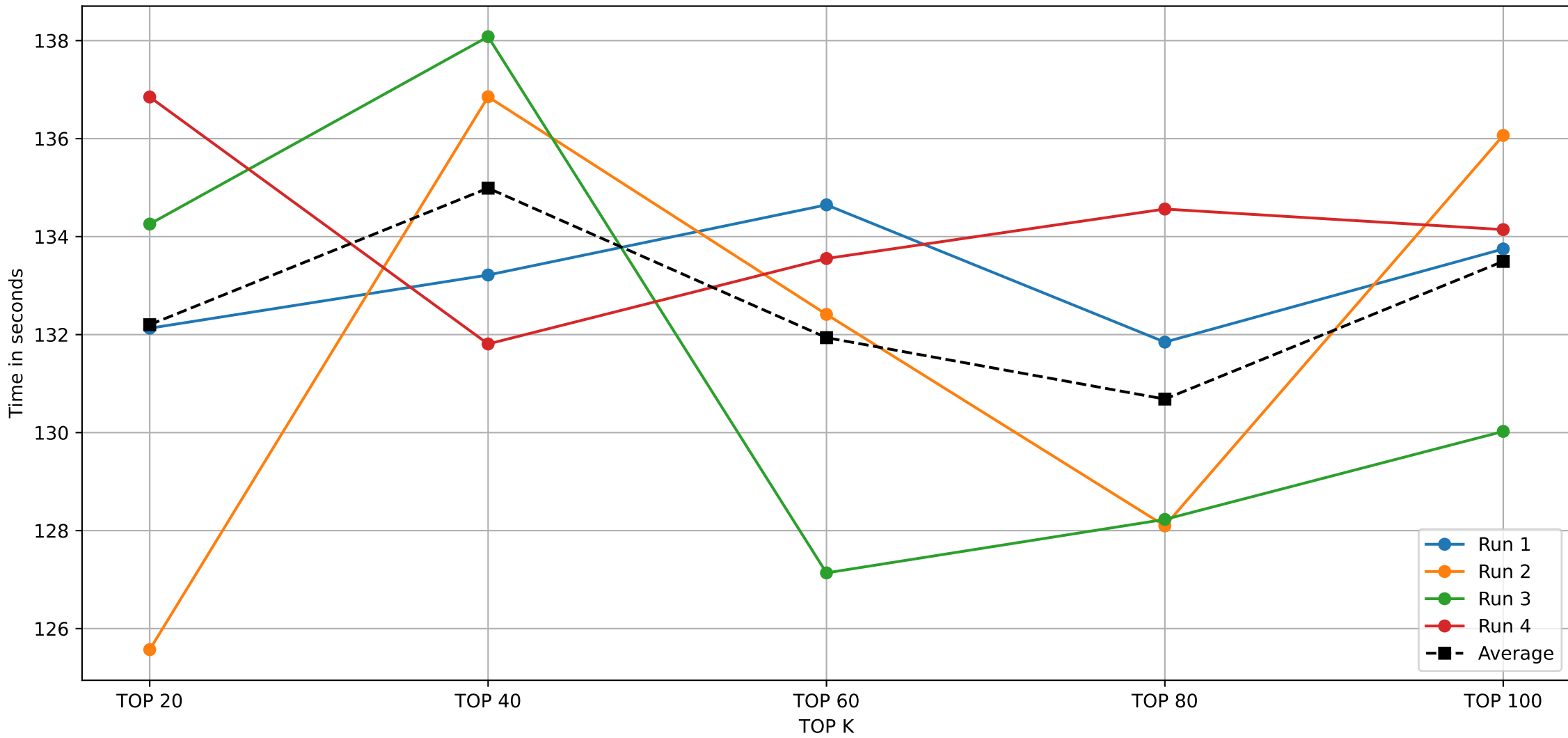
NAIVE ALGORITHM ON 1000000 TRANSACTIONS DATABASE
