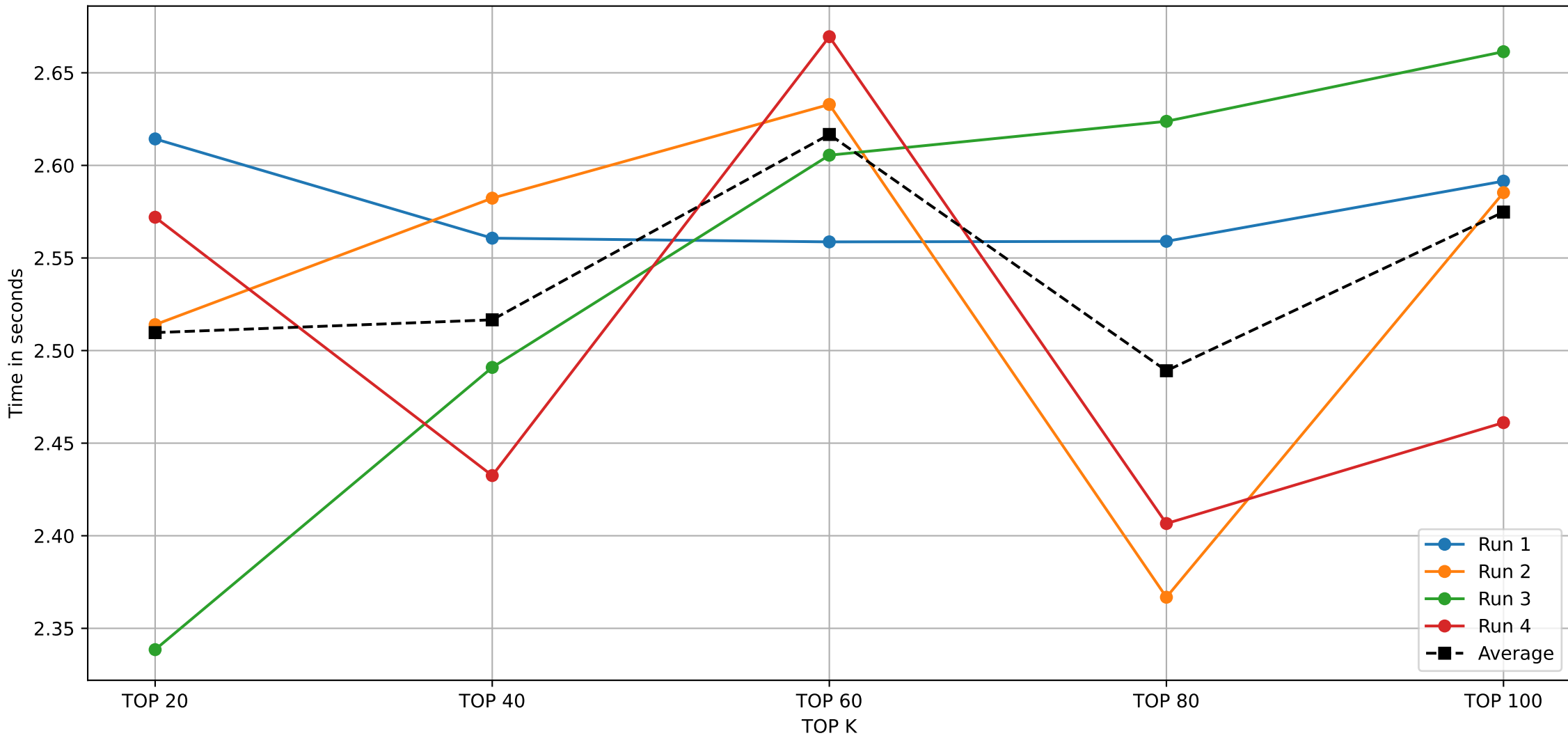
HEURISTIC ALGORITHM ON 20000 TRANSACTIONS DATABASE
