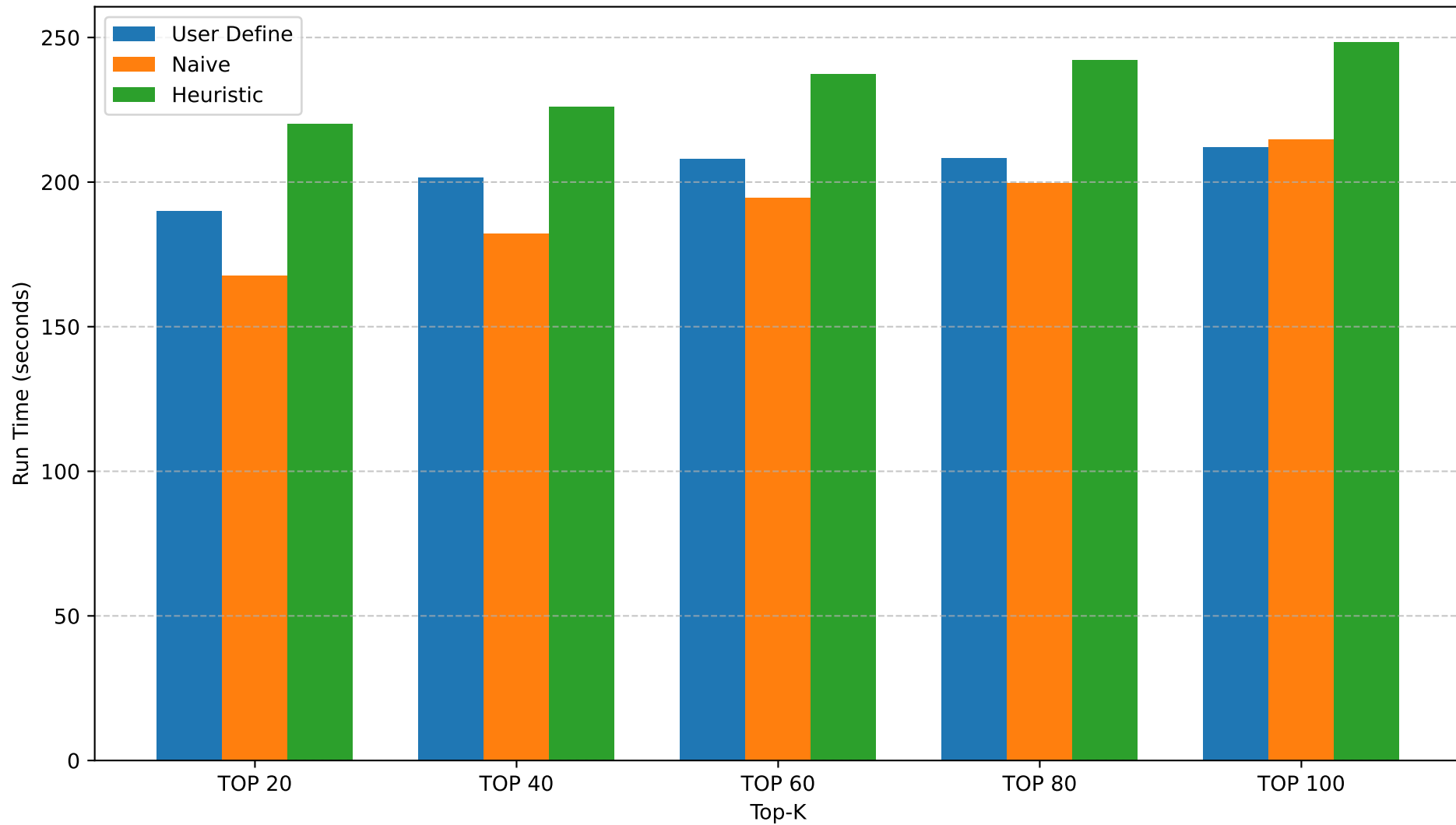
Run Time Comparison (2,000,000 Transactions)
