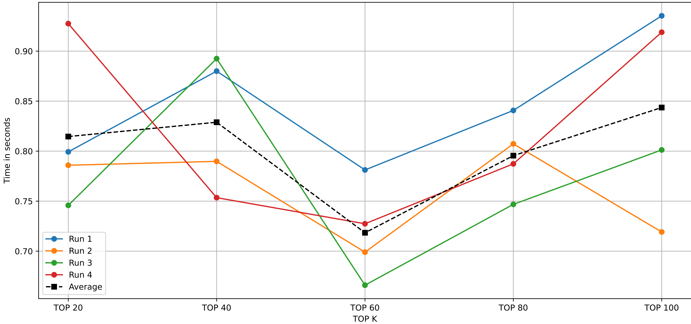
NAIVE ALGORITHM ON 10000 TRANSACTIONS DATABASE
