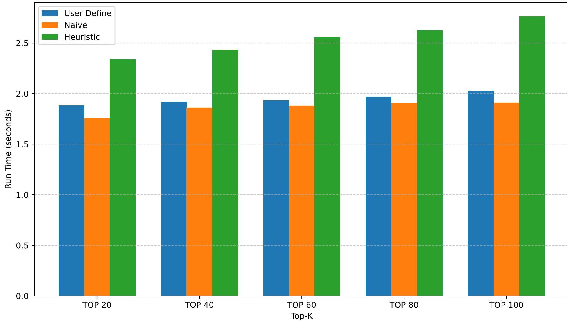
Run Time Comparison (20,000 Transactions)
