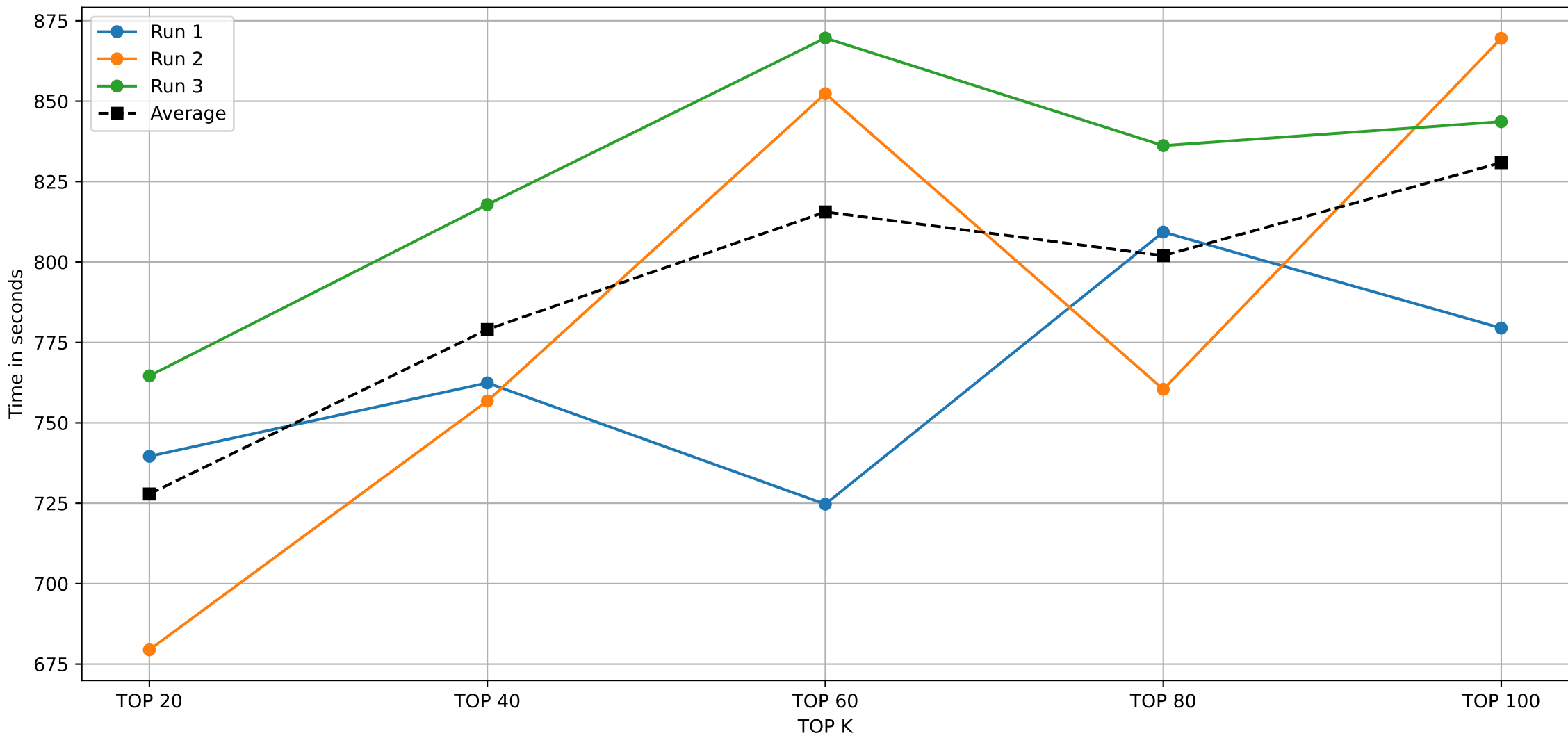
NAIVE ALGORITHM ON 5000000 TRANSACTIONS DATABASE
