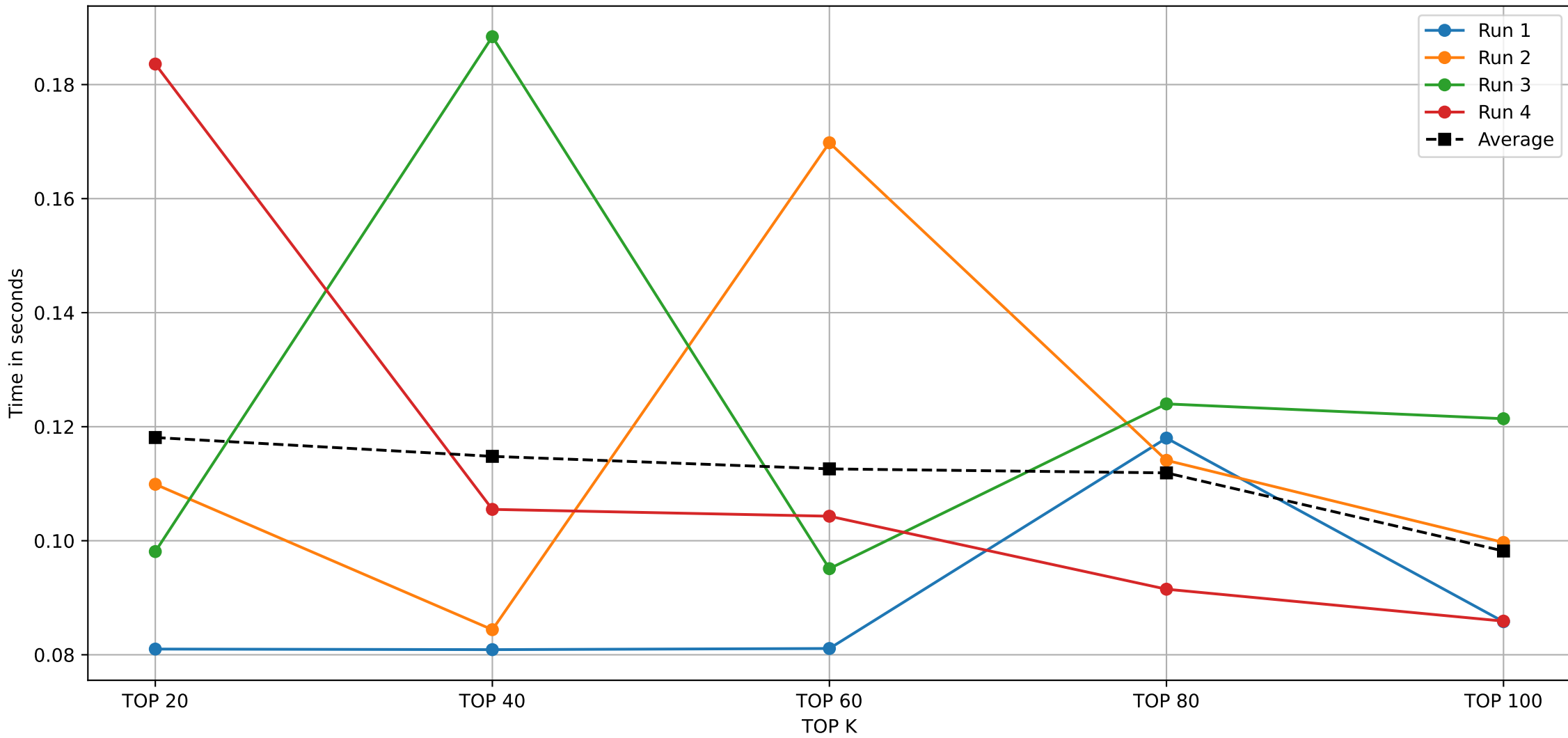
NAIVE ALGORITHM ON 2000 TRANSACTIONS DATABASE
