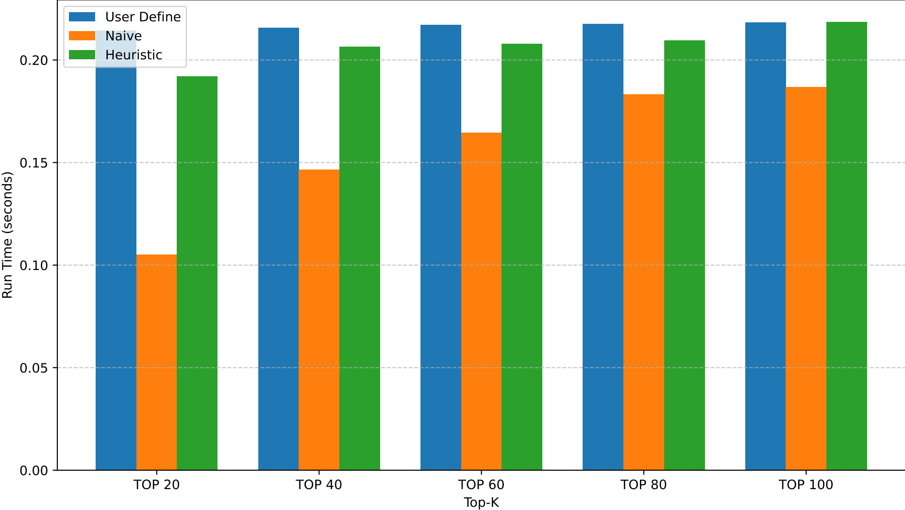
Run Time Comparison (5000 Transactions)
