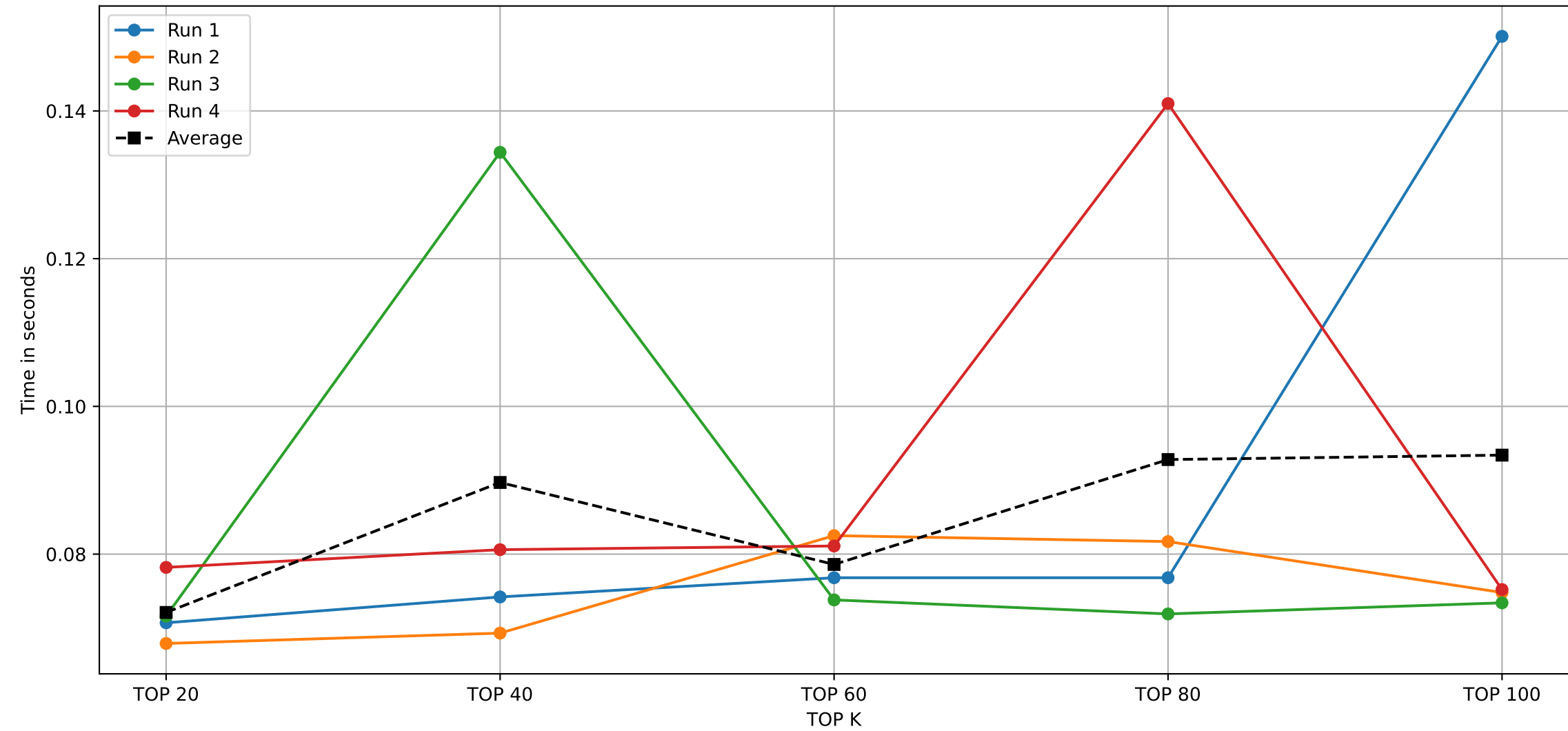
NAIVE ALGORITHM ON 1000 TRANSACTIONS DATABASE
