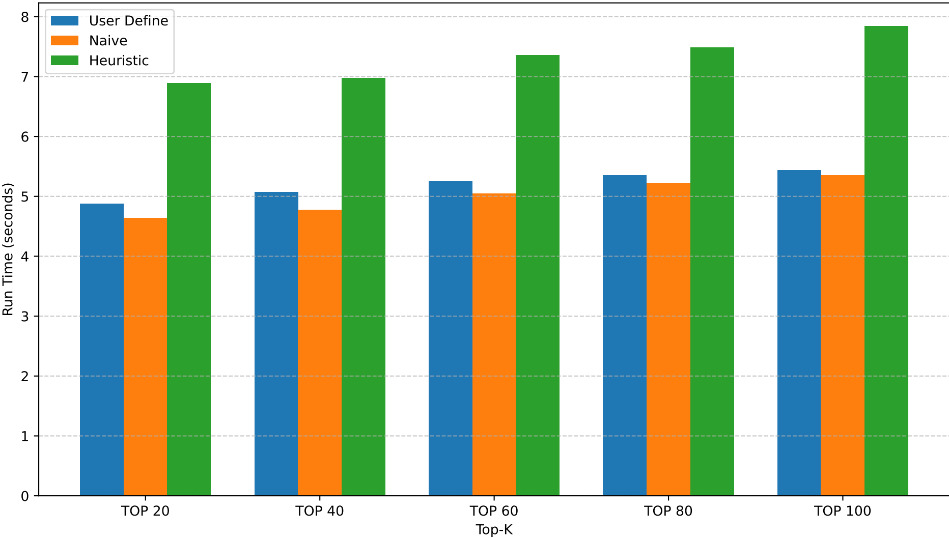
Run Time Comparison (50,000 Transactions)
