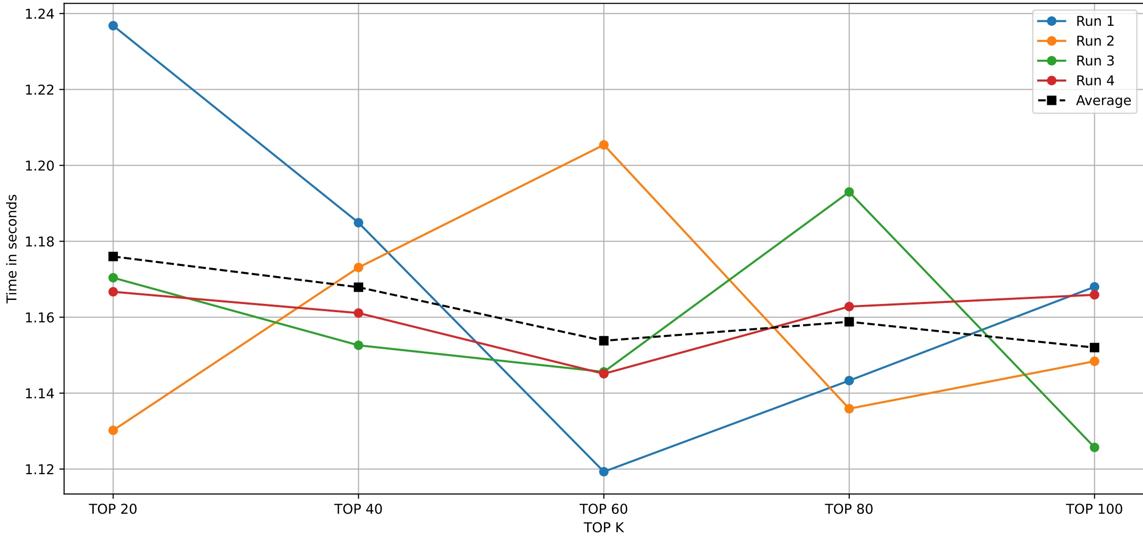
HEURISTIC ALGORITHM ON 10000 TRANSACTIONS DATABASE
