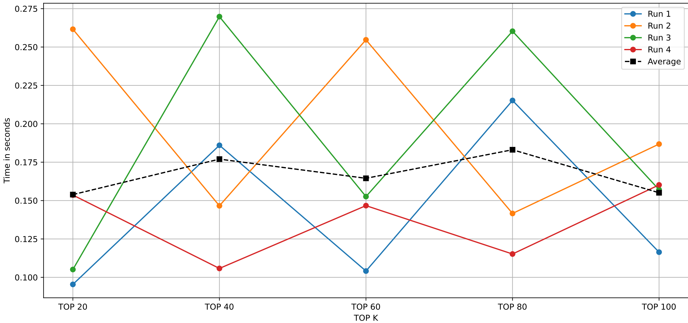
NAIVE ALGORITHM ON 5000 TRANSACTIONS DATABASE
