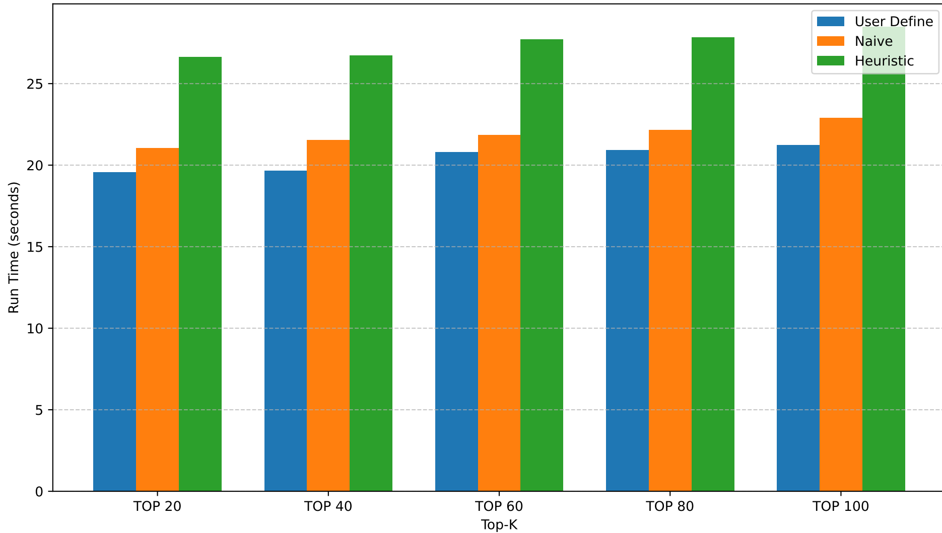
Run Time Comparison (200,000 Transactions)
