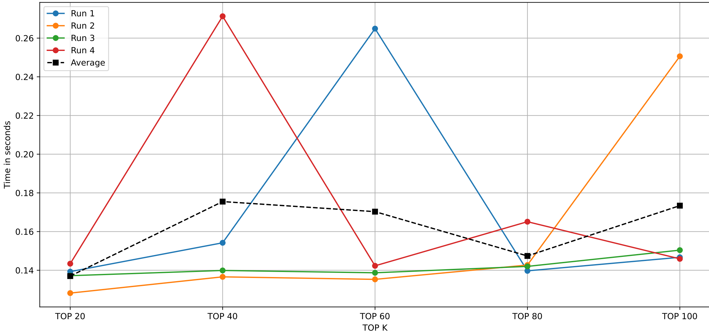
HEURISTIC ALGORITHM ON 1000 TRANSACTIONS DATABASE
