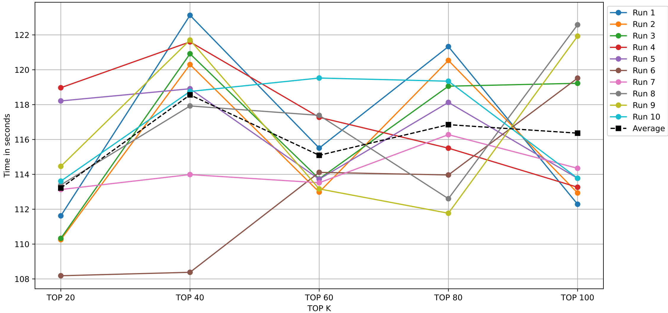
USER DEFINE ALGORITHM ON 1,000,000 TRANSACTIONS DATABASE
