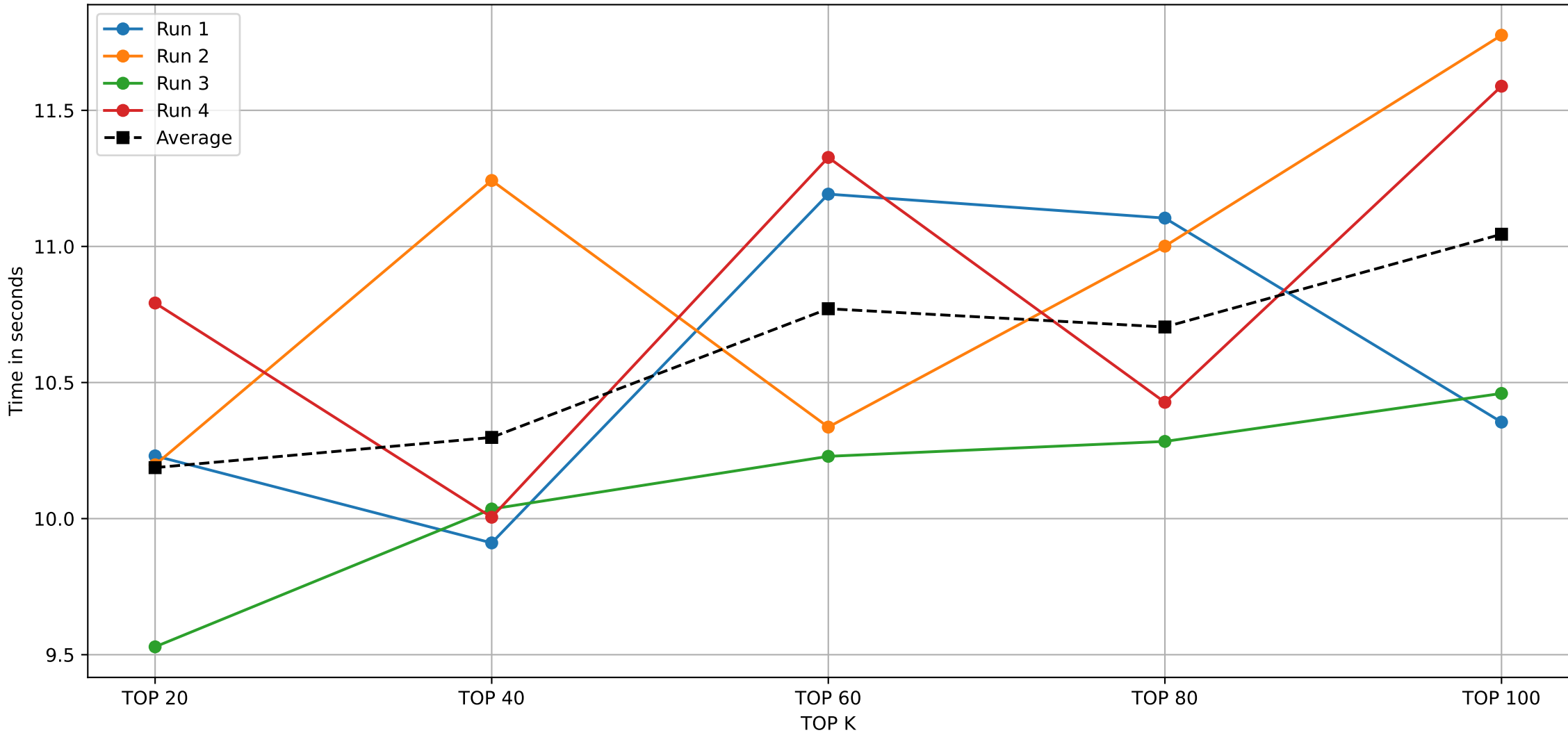
NAIVE ALGORITHM ON 100000 TRANSACTIONS DATABASE
