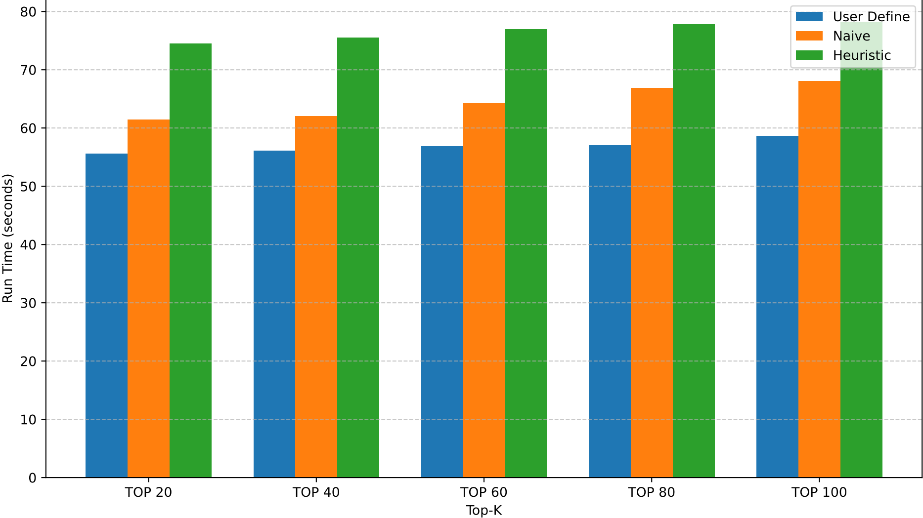
Run Time Comparison (500,000 Transactions)
