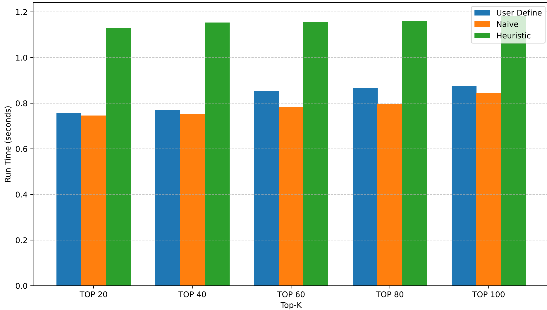
Run Time Comparison (10,000 Transactions)
