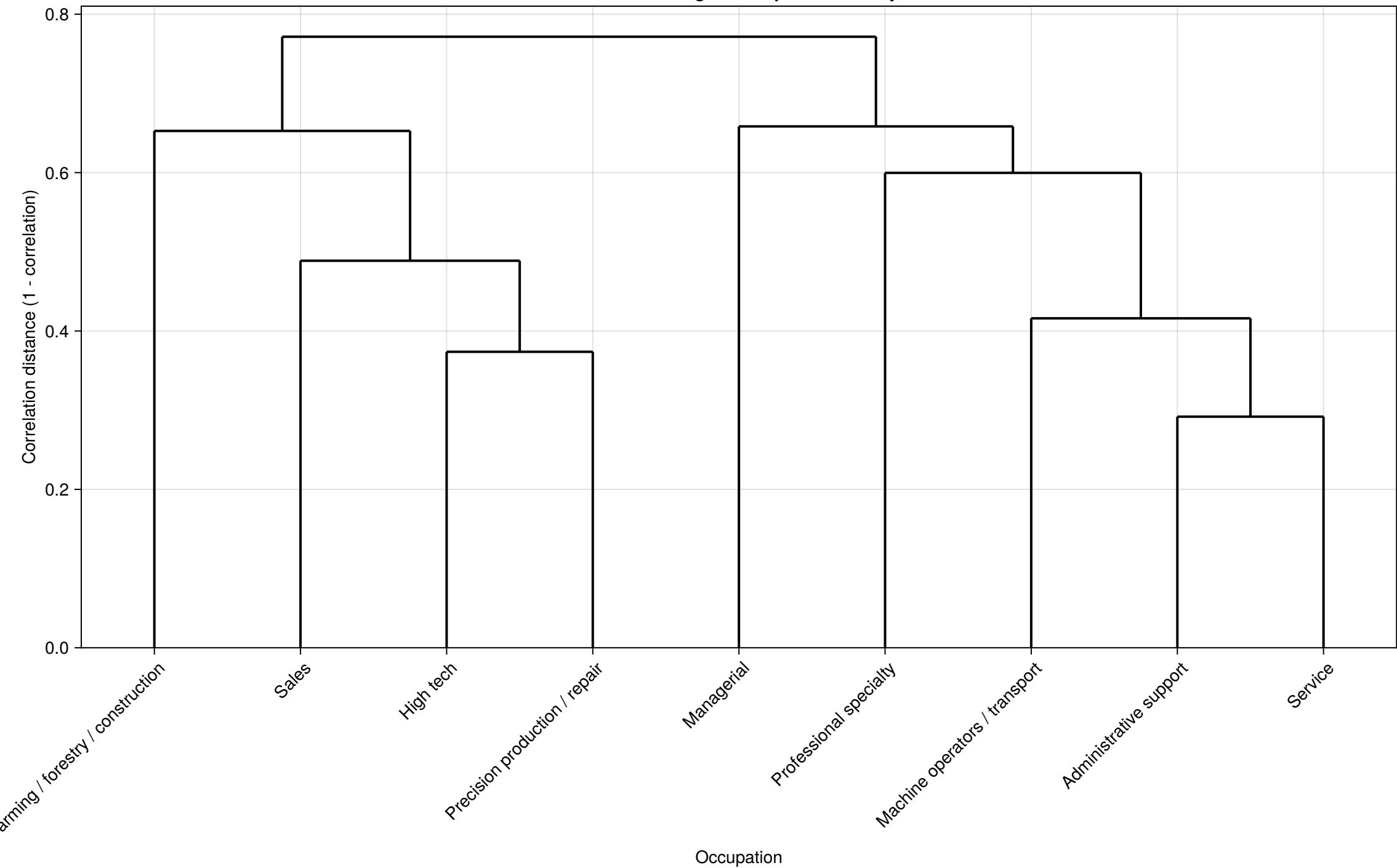
Hierarchical Clustering of Occupation IRF Trajectories
