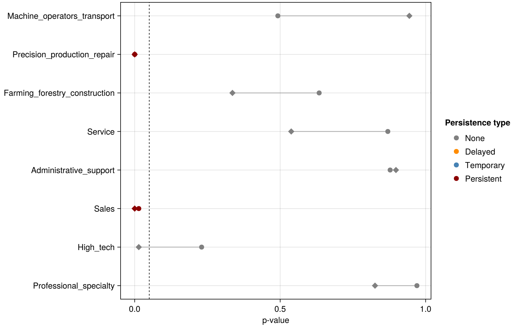
Persistence Classification: Response of Log Income
