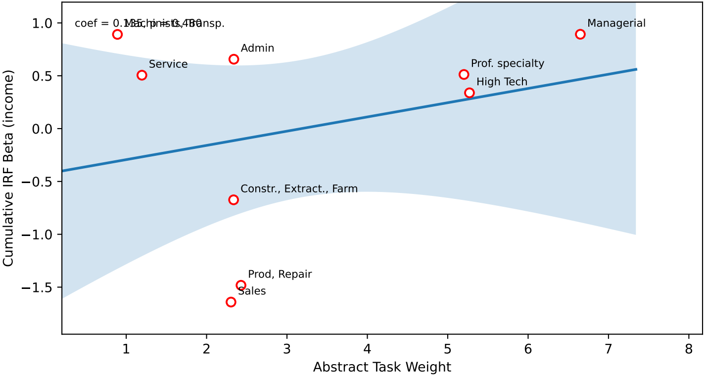
Task Characteristics vs Cumulative IRF: income
