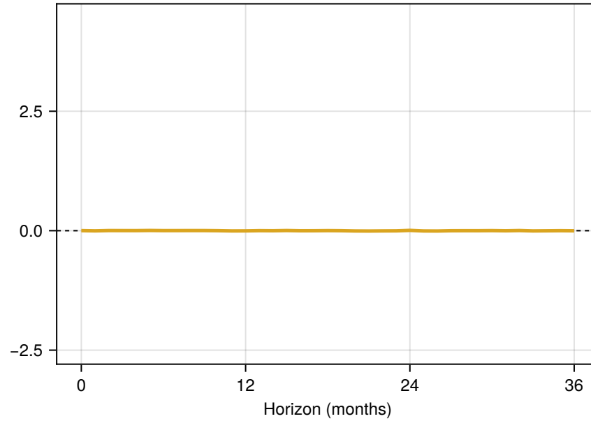
(9) Machine_ops_transport
