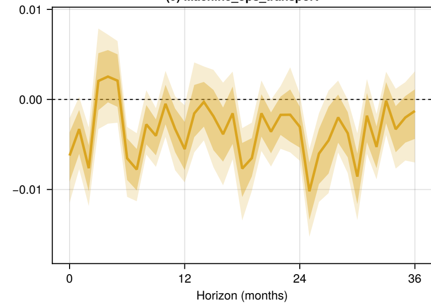
(9) Machine_ops_transport
