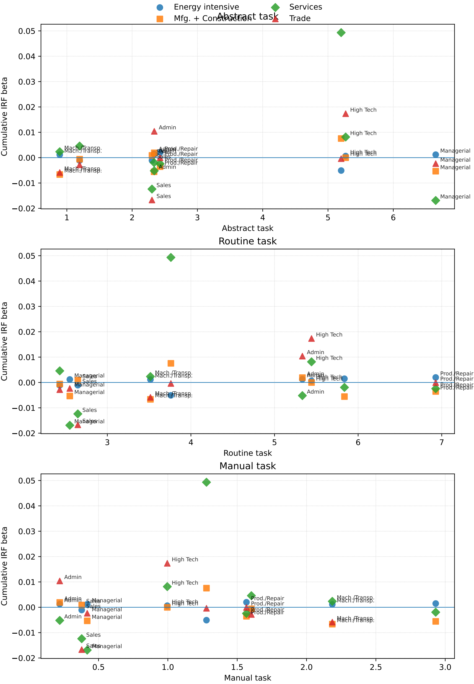
Raw task relationships by industry: income_share_var
