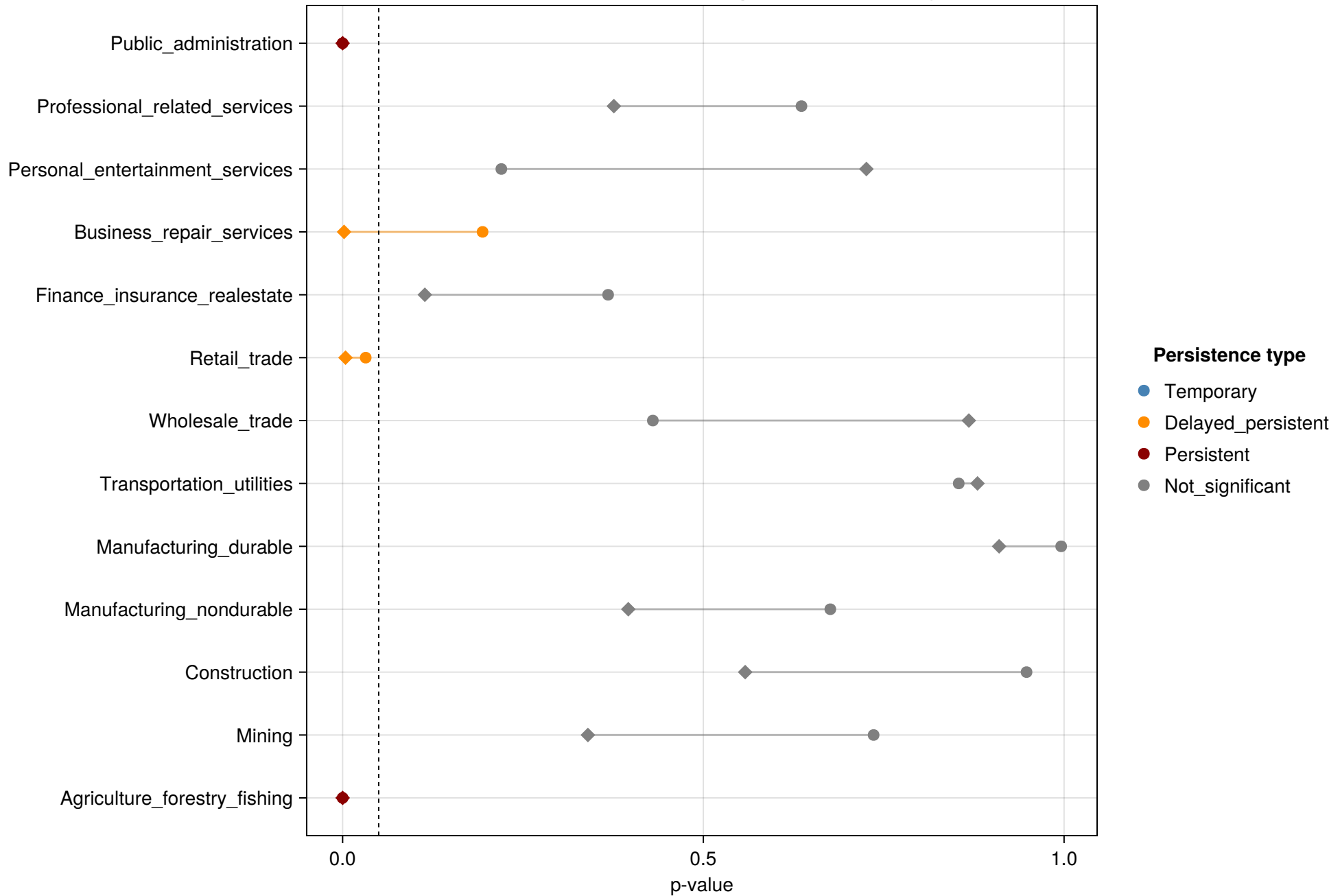
Persistence Classification: Response of Median Wage
