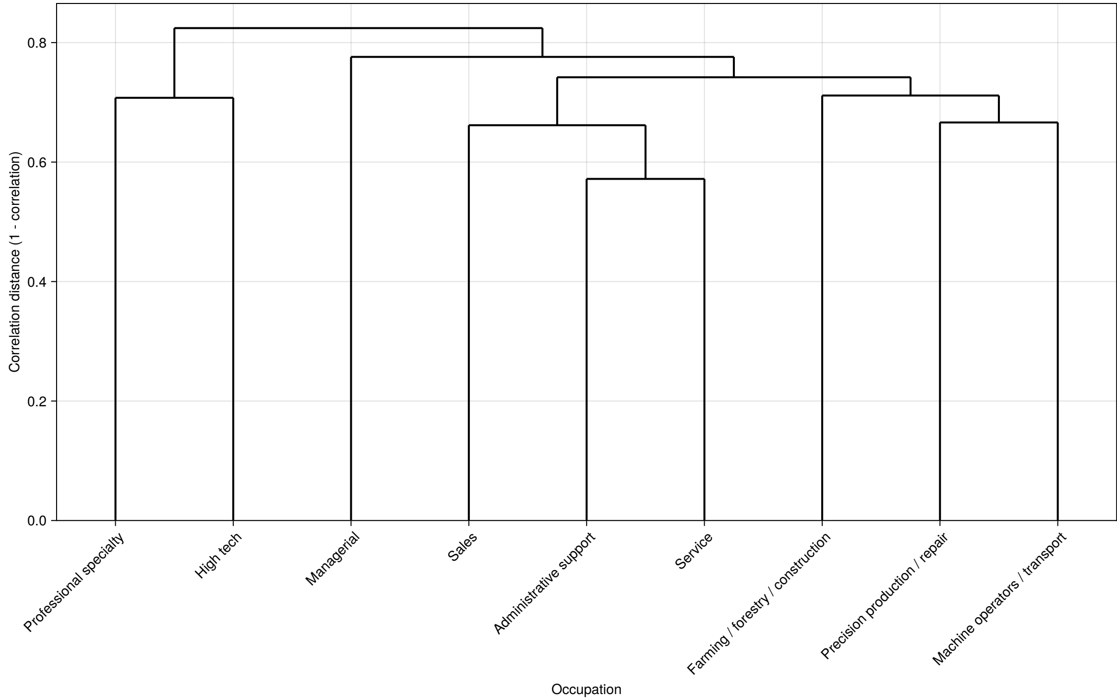
Hierarchical Clustering of Occupation IRF Trajectories
