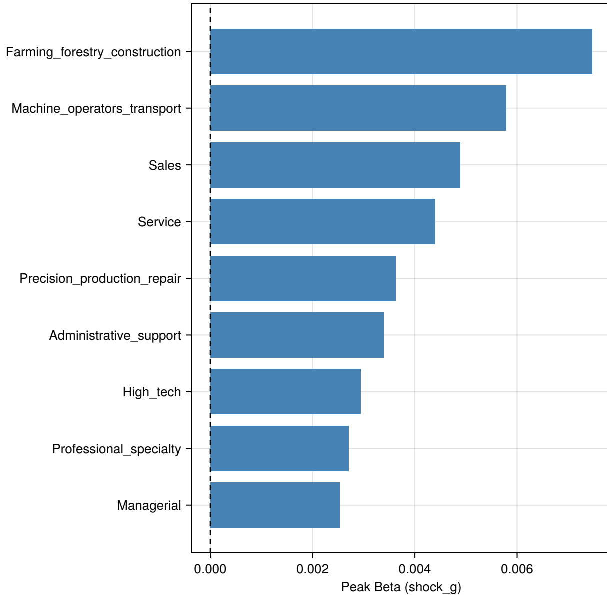
Peak IRF Response — unemployment
